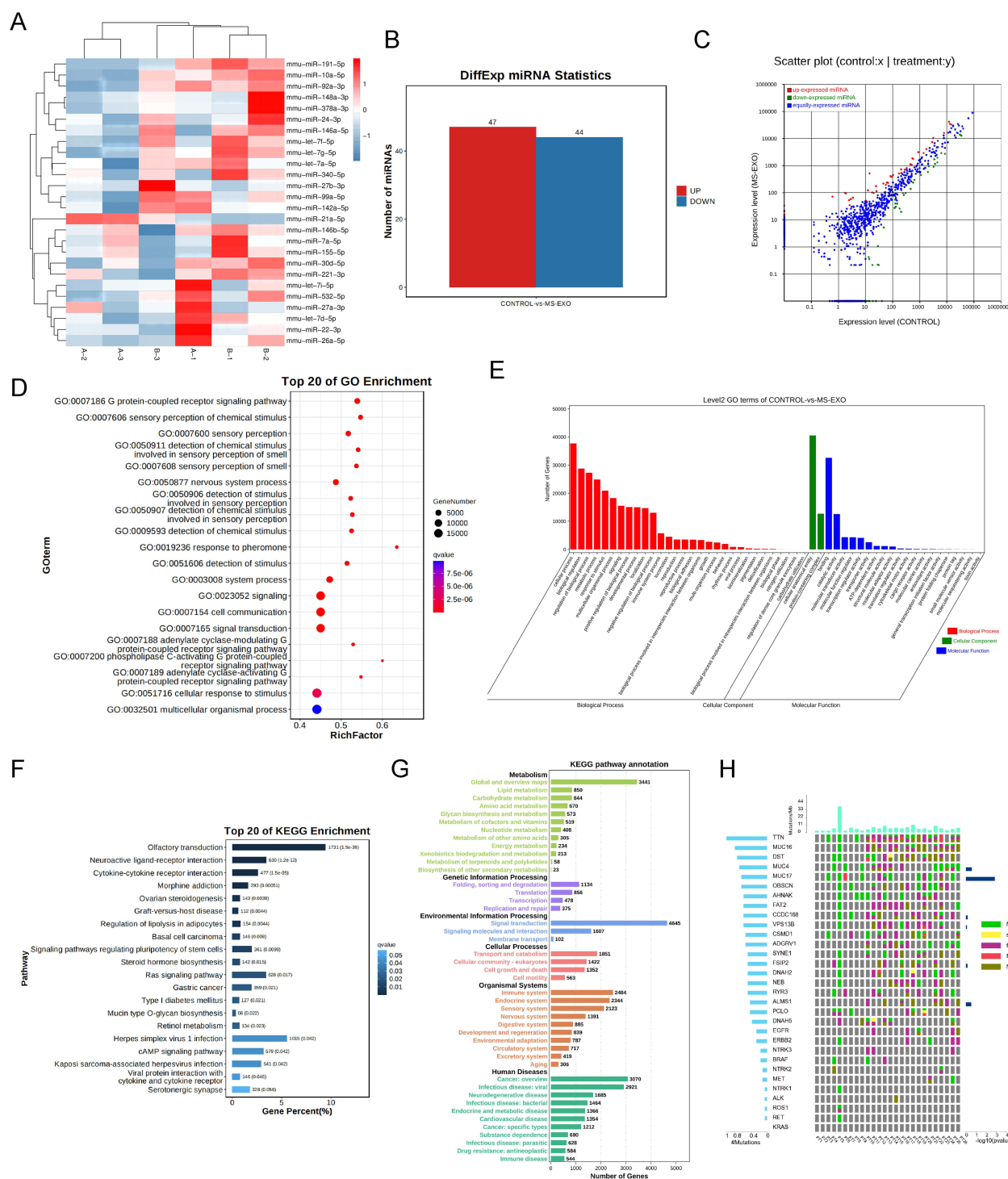
Figure 4 Functional attributes related to changes in gene sets and signaling pathways induced by Exosome-MS were analyzed. (A) A heat map was generated to depict the differential expression of miRNAs. (B) MiRNAs that were both upregulated and downregulated were identified. (C) A scatter plot was utilized to illustrate both the upregulated and downregulated miRNAs. (D) The genes were classified based on the biological processes using GO classification. (E) GO enrichment diagram shows the main gene function classification. (F) The related signaling pathways were evaluated through the utilization of KEGG pathway analysis. (G) The differentially expressed genes were classified into different groups based on the metabolic pathways using KEGG analysis. (H) Differential miRNA chromosomal localization between Exosome and Exosome-MS.
