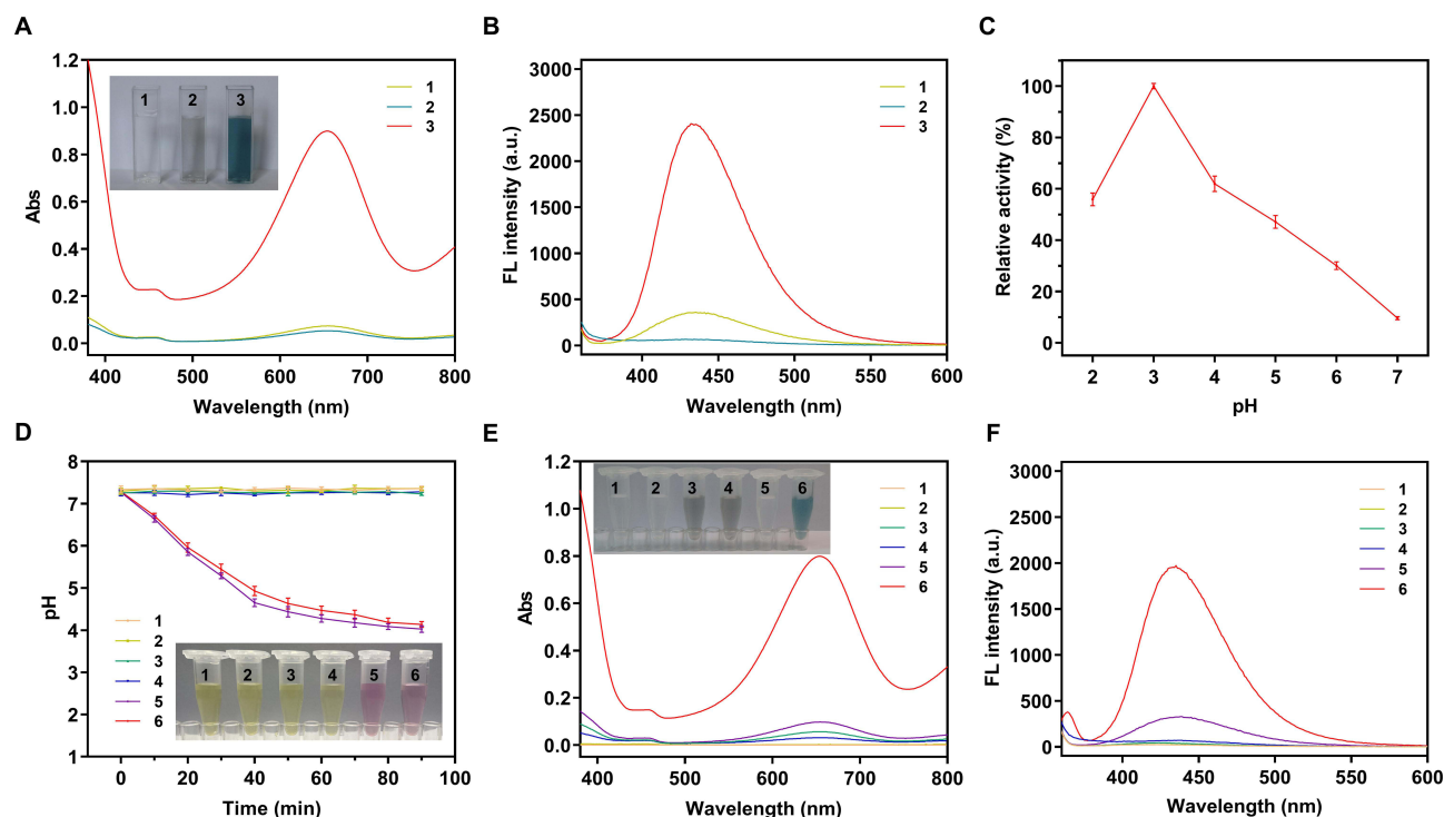
Figure 2 (A) UV-vis spectra and photographs of different reaction systems: (1) \text{H}_2\text{O}_2 + TMB, (2) HMMo-SAzyme + TMB, and (3) HMMo-SAzyme + \text{H}_2\text{O}_2 + TMB. (B) Fluorescence spectra of different reaction systems: (1) \text{H}_2\text{O}_2 + TA, (2) HMMo-SAzyme + TA, and (3) HMMo-SAzyme + \text{H}_2\text{O}_2 + TA. (C) Peroxidase-like activity of HMMo-SAzyme at different pH values. Data are shown as mean \pm SD. (D) pH value versus reaction time under different reaction systems; insets are the corresponding photographs in the presence of methyl red. Data are shown as mean \pm SD. (E) UV-vis spectra and photographs of different reaction systems in the presence of TMB. (F) Fluorescence spectra of different reaction systems in the presence of TA. Different reaction systems in (D–F): (1) PBS, (2) glucose, (3) HMMo/GOx, (4) glucose + HMMo-SAzyme, (5) glucose + GOx, (6) glucose + HMMo/GOx.
