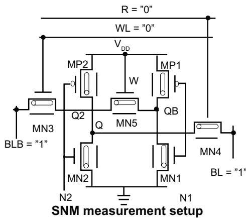
Figure 9 Test setup for measuring static noise margin (SNM).
