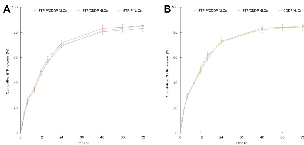
Figure 4 In vitro release of Etp (A) and CDDP (B) from NLCs was analyzed using dialysis. NLCs (2 mL) were put in a dialysis bag, immersed in 100 mL PBS in the presence of 10% FBS (pH 7.4), and placed on a shaking bed at 37°C with a rotation speed of 100 rpm. Note: Data presented as means \pm SD, n=6.
