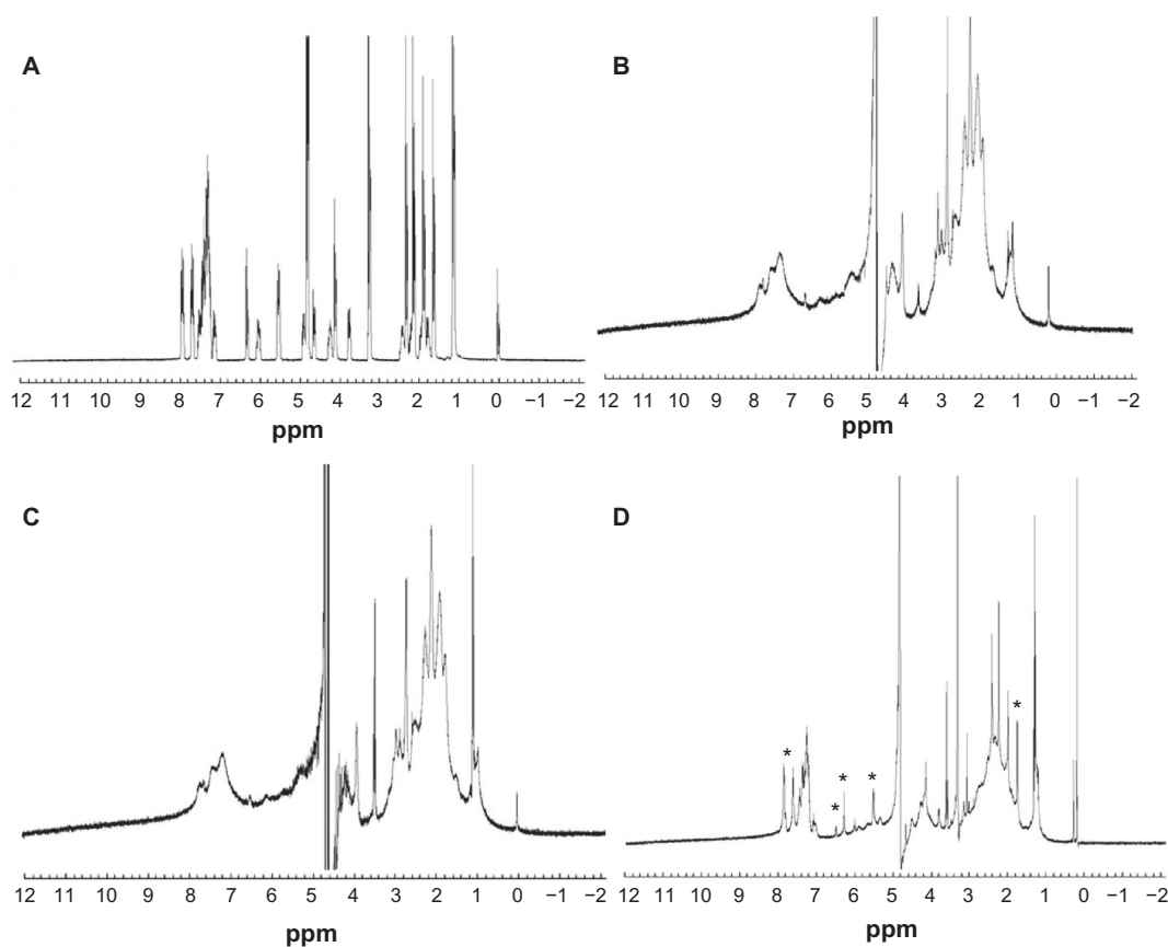
Figure 2 A) ^1\text{H-NMR} spectra of paclitaxel in \text{CD}_3\text{OD} ; B) PGG-PTX nanoconjugate in \text{D}_2\text{O} ; C) paclitaxel-loaded PGG-PTX nanoparticles in \text{D}_2\text{O} ; and D) paclitaxel-loaded PGG-PTX nanoparticles in \text{CD}_3\text{OD} .
