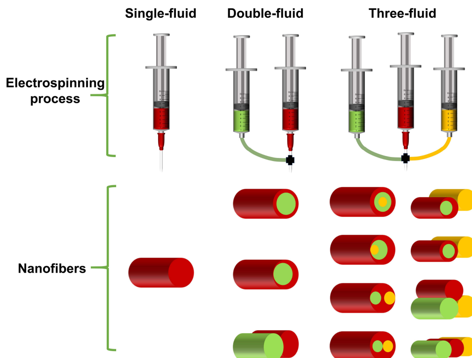
Figure 4 Schematic diagram of the electrospinning process classification and their respective fiber structure.
