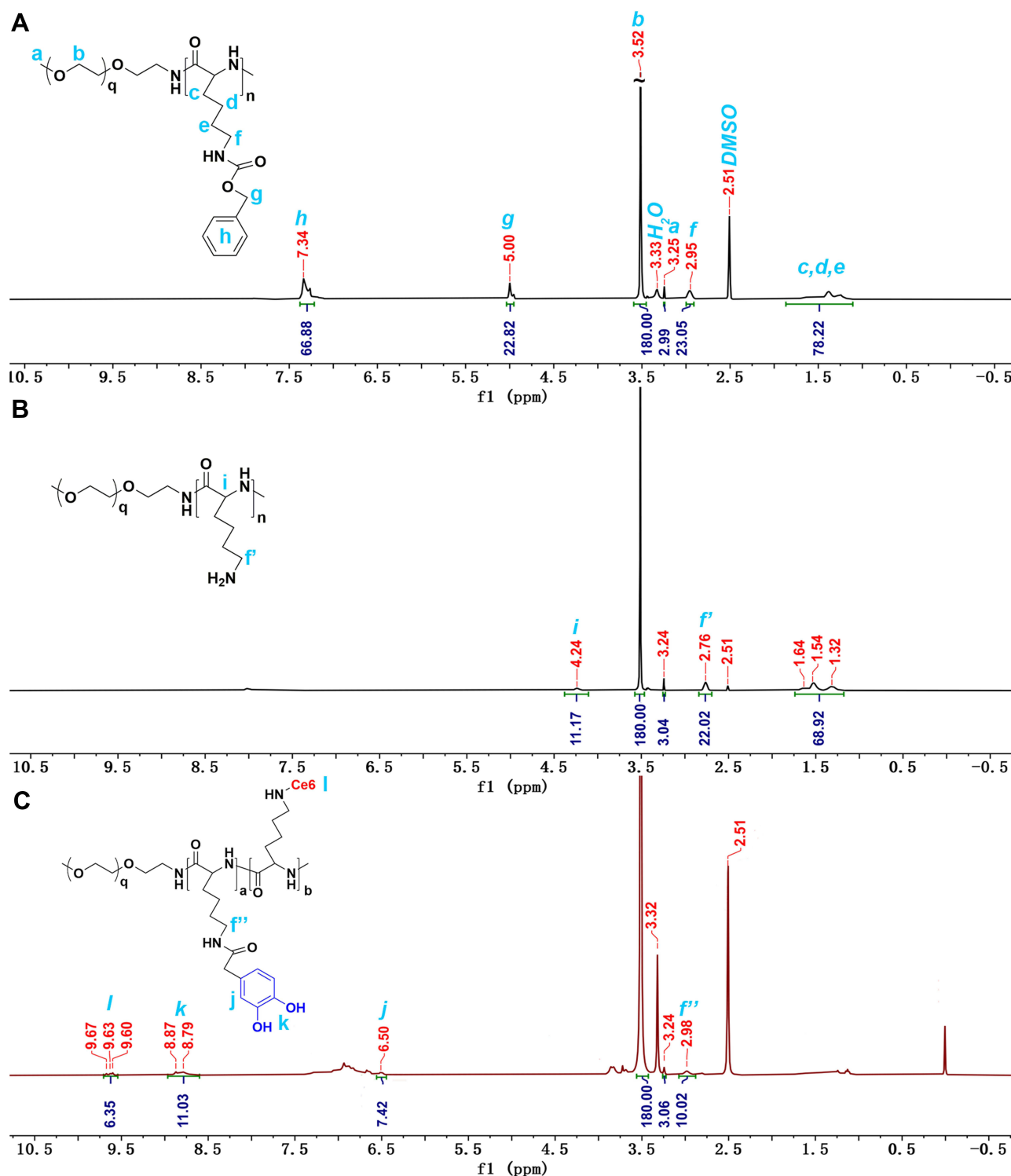
Figure 1 ^1\text{H-NMR} (500 MHz) of (A) mPEG-Plys (Z), (B) mPEG-Plys, and (C) mPEG-Plys (DA-Ce6) in \text{DMSO-d}_6 .
