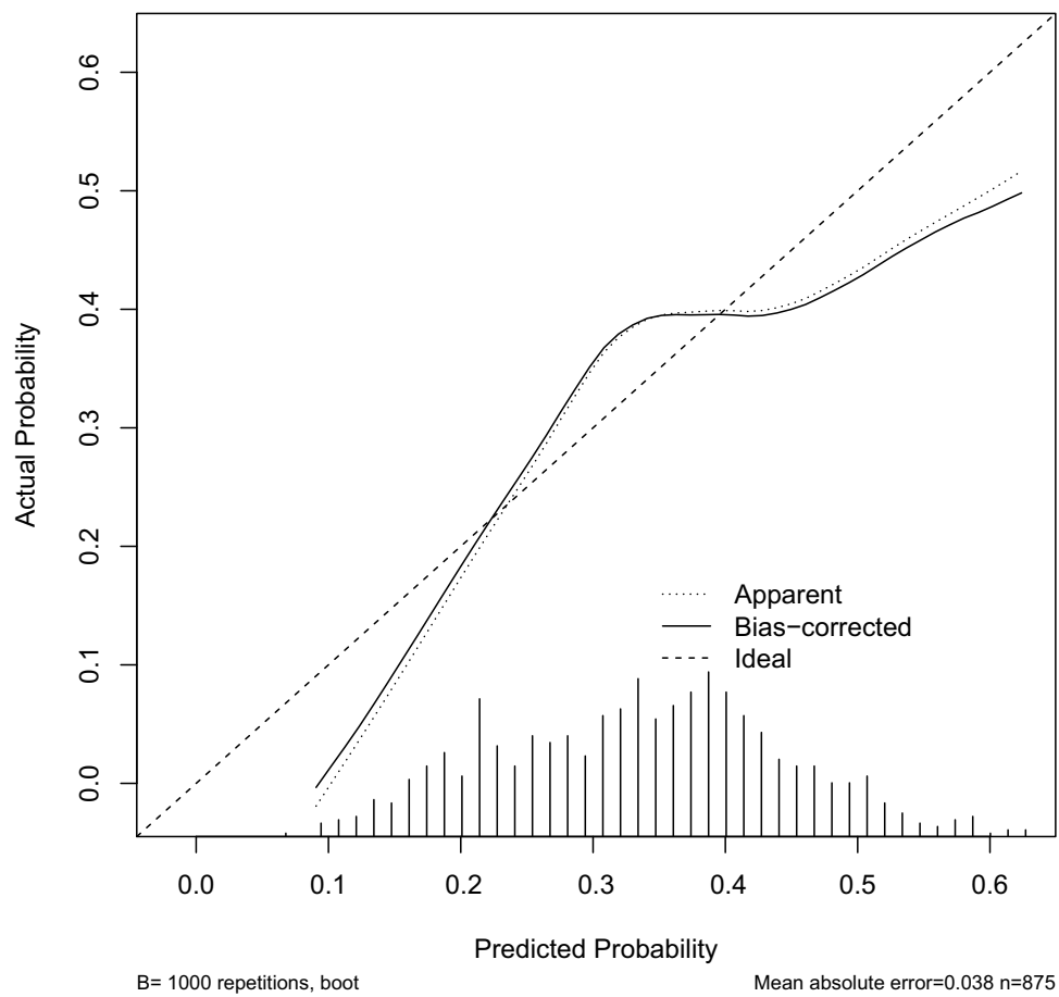
Figure 3 Calibration plots of the nomogram.
