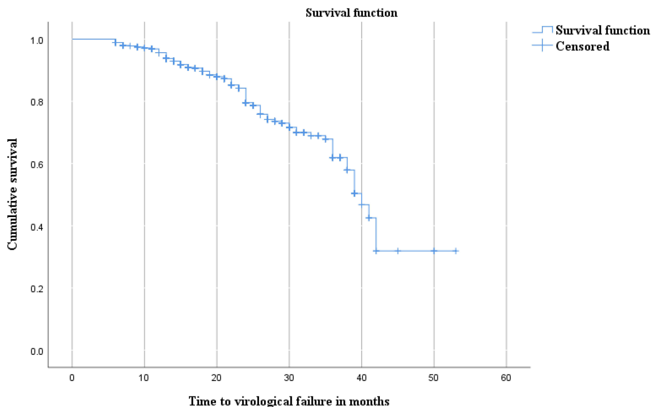
Figure 3 Kaplan Meier curve analysis of virological treatment failure starting from six months of follow-up.
