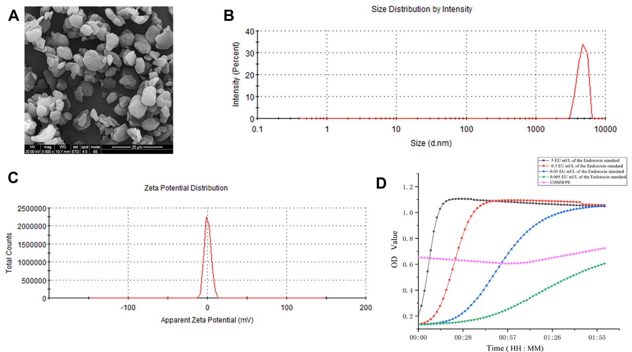
Figure 1 Characterization of UHMWPE microparticles. (A) SEM image showing the shape and size distribution of the UHMWPE microparticles. Scale bar: 20 μm. (B and C) The size distribution and zeta potential of UHMWPE microparticles were analyzed using DLS. (D) Curve showing the endotoxin concentration in UHMWPE.
