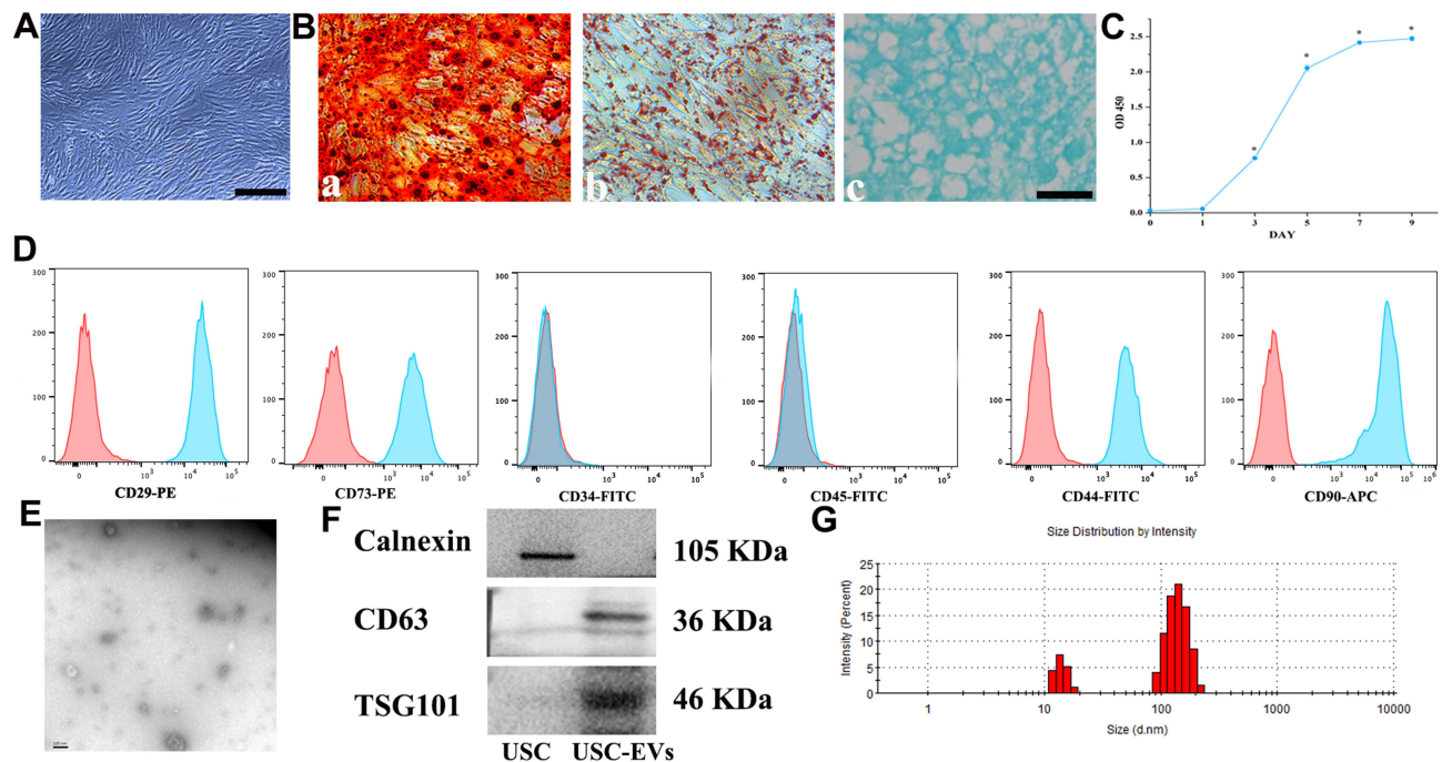
Figure 2 Characterization of USCs and USC-EVs. (A) The morphology of USCs. Scale bar: 100 μm. (B-a) Osteogenic differentiation of USCs determined using Alizarin Red S staining. Scale bar: 100 μm. (B-b) Adipogenic differentiation of USCs determined using Oil Red O staining. Scale bar: 100 μm. (B-c) Chondrogenic differentiation of USCs determined using Alcian Blue staining. Scale bar: 100 μm. (C) USCs growth curve. (D) MSC surface markers in USCs determined by flow cytometry analysis. (E) Transmission electron microscopy image of USC-EVs. Scale bar: 100 nm. (F) Typical surface markers expressed on USC-EVs and USCs determined by Western blot analysis. (G) USC-EV size distribution measured using DLS analysis. *P<0.05.
