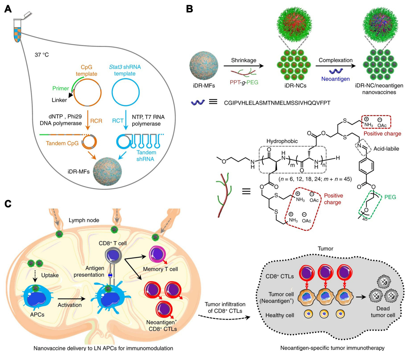
Figure 4 The iDR-NC/neoantigen nanovaccines constructed by DNA self-assembly loaded with CpG. (A) Tandem CpG and shRNAs were produced through RCR and RCT, and self-assembled into intertwining DNA-RNA MFs. (B) The above-mentioned MFs were contracted by PPT-g-PEG into iDR-NCs, which were further loaded with tumor neoantigens. (C) Specific anti-tumor response induced by iDR-NCs/neoantigen nanovaccines in mice. Adapted from Zhu G, Mei L, Vishwasrao HD, et al. Intertwining DNA-RNA nanocapsules loaded with tumor neoantigens as synergistic nanovaccines for cancer immunotherapy. Nat Commun. 2017;8(1):1482. 100
