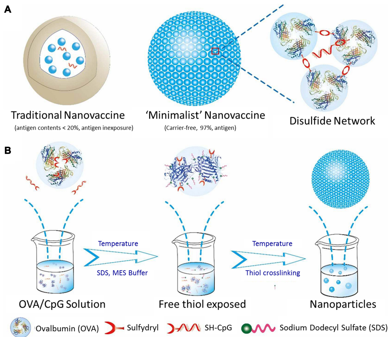
Figure 3 Design of "minimalist" OVA@CpG nanovaccine. (A) Traditional nanovaccine and "minimalist" nanovaccine. (B) The general process of constructing the "minimalist" nanovaccine. Adapted with permission from Wang K, Wen S, He L, et al. "Minimalist" nanovaccine constituted from near whole antigen for cancer immunotherapy. ACS Nano . 2018;12(7):6398–6409. Copyright 2018 American Chemical Society. 85
