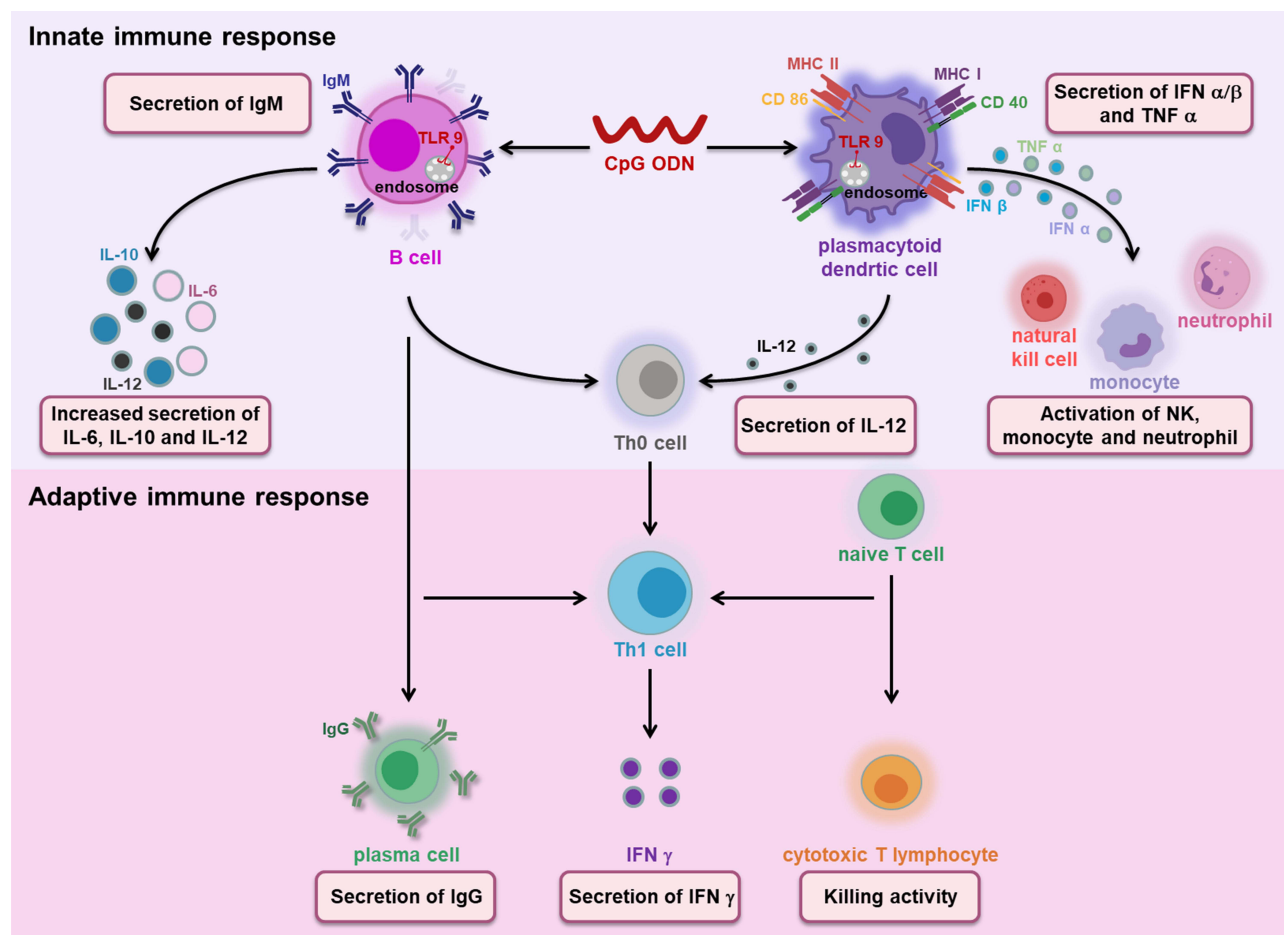
Figure 1 The mechanism of CpG ODN inducing innate and adaptive immune response.
