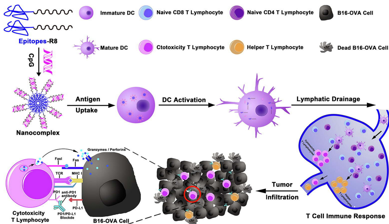
Figure 2 Schematic of the nanocomplex vaccine and specific anti-tumor T cell immune response. The nanovaccine was formed by co-assembly of the adjuvant CpG and the cationic Epitopes-R8. Reprinted from Chemical Engineering Journal, 399, Shi X, Song H, Wang C, et al, Co-assembled and self-delivered epitope/CpG nanocomplex vaccine augments peptide immunogenicity for cancer immunotherapy, 125854, Copyright 2020, with permission from Elsevier. 81
