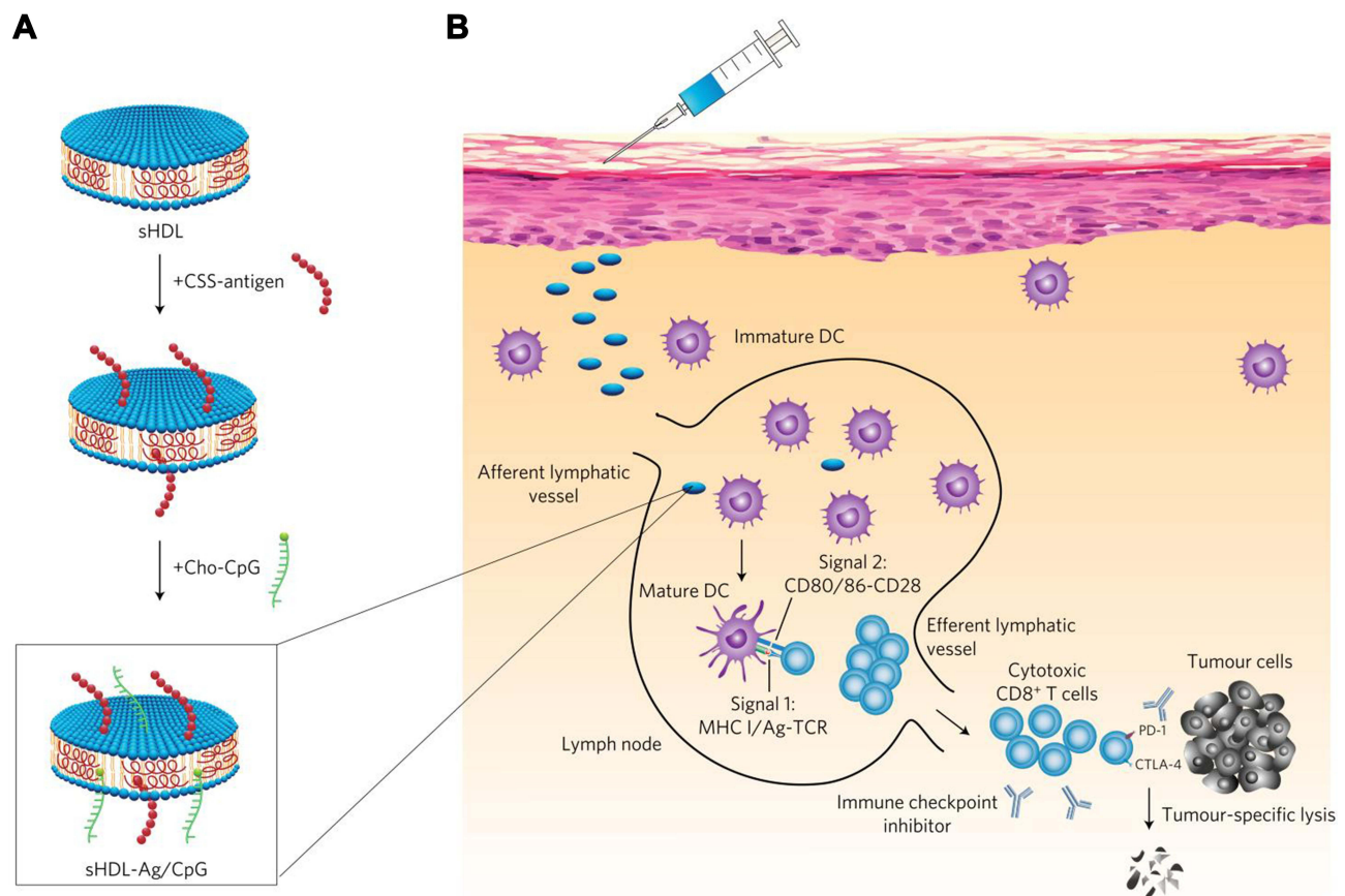
Figure 5 Construction of sHDL nanodisk platform for personalized vaccines for cancer immunotherapy. (A) The binding process of antigen and adjuvant CpG into sHDL nanodisk platform. (B) The designed personalized nanovaccines could induce a strong CTL response in vivo. Reprinted by permission from Springer Nature Customer Service Centre GmbH: Springer Nature, Nature Materials. Kuai R, Ochyl LJ, Bahjat KS, Schwendeman A, Moon JJ. Designer vaccine nanodiscs for personalized cancer immunotherapy. Nat Mater . 2017;16(4):489–496. doi:10.1038/nmat4822. Copyright 2017. 104
