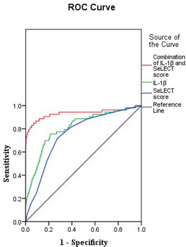
Figure 1 ROC curves of IL-1 \beta , SeLECT score and their combination in predicting PSE.
