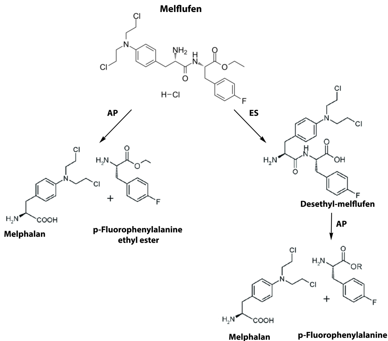
Figure 1 Chemical structure and metabolism of melflufen (melflufen flufenamide) hydrochloride, a dipeptide prodrug of melflufen. Melflufen is metabolized into melflufenamide and p-Fluorophenylalanine by aminopeptidases (AP) inside myeloma cells. Melflufen utilizes not only intracellular aminopeptidases (AP) but also esterases (ES) to release a melflufen cytotoxic payload in neoplastic myeloma cells.
