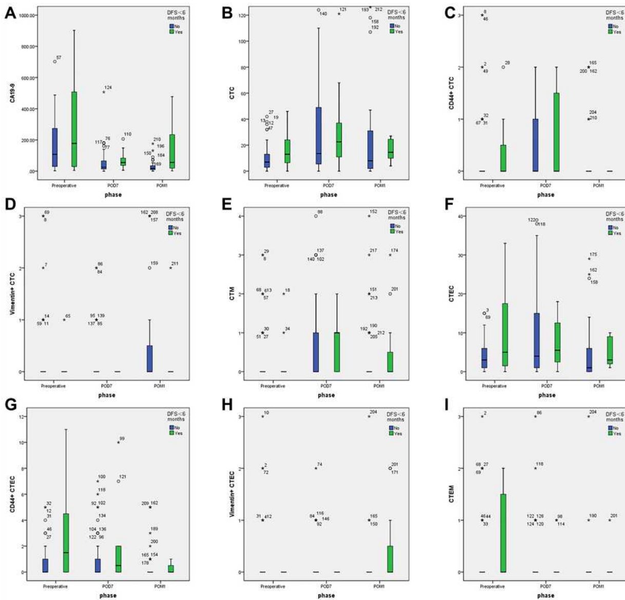
Figure 3 The dynamics of (A) CA 19-9 levels, numbers of (B) CTCs, (C) CD44+ CTC, (D) vimentin+ CTC, (E) CTCM, and numbers of (F) CTECs (G) CD44+ CTEC, (H) vimentin+ CTEC, (I) CTEM in different phases (preoperative, POD7 and POM1). The patients were divided into early recurrence (ER) group (DFS<6 months) and late recurrence (LR) group (DFS≥6 months) according to the DFS.
