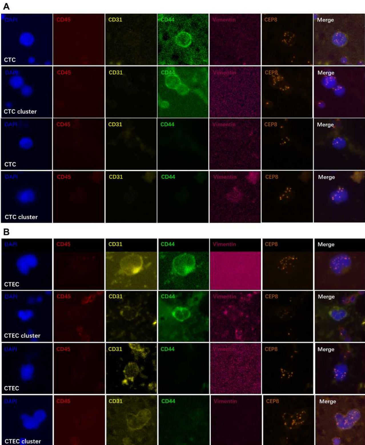
Figure 1 Detection of different subtypes of CTCs and CTECs expressing CD44 and vimentin in PDAC patients by SE-iFISH. (A) A CTC (DAPI+/CD45-/CD31-/vimentin-/CEP8+) has a positive expression of CD44; A CTC cluster (DAPI+/CD45-/CD31-/vimentin-/CEP8+) has a positive expression of CD44; A CTC (DAPI+/CD45-/CD31-/vimentin-/CEP8+) has a negative expression of CD44; A CTC cluster (DAPI+/CD45-/CD31-/vimentin+/CEP8+) has a negative expression of CD44. (B) A CTEC (DAPI+/CD45-/CD31+/vimentin-/CEP8+) has a positive expression of CD44; A CTEC cluster (DAPI+/CD45-/CD31+/vimentin+/CEP8+) has a positive expression of CD44; A CTEC (DAPI+/CD45-/CD31+/vimentin-/CEP8+) has a negative expression of CD44; A CTEC cluster (DAPI+/CD45-/CD31+/vimentin+/CEP8+) has a negative expression of CD44.
