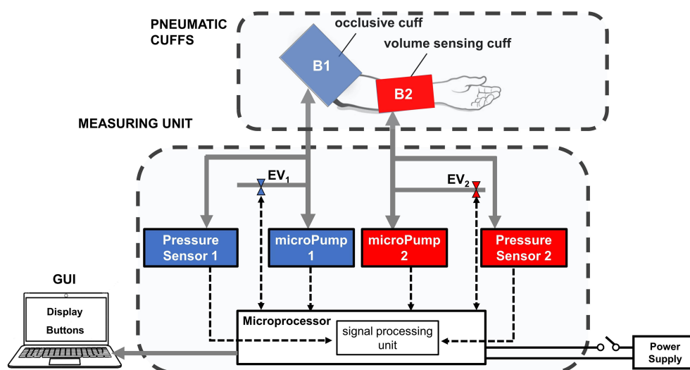
Figure 2 Block diagram of the main components of VenCoM device.
