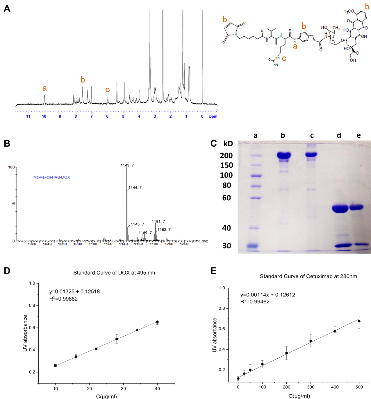
Figure 3 (A) ^1\text{H} -NMR (DMSO) analysis of MC-Val-Cit-PAB-DOX. (B) Mass spectrometry results of MC-Val-Cit-PAB-DOX. (C) SDS-PAGE analysis of (a) protein marker, (b) cetuximab, (c) cetuximab-vc-DOX, (d) cetuximab treated with \beta -mercaptoethanol, (e) cetuximab-vc-DOX treated with \beta -mercaptoethanol. (D) Standard curves of DOX (10–40 \mu\text{g/mL} ) at 495 nm. (E) Standard curves of the monoclonal antibody (5–1500 \mu\text{g/mL} ) at 280 nm.
