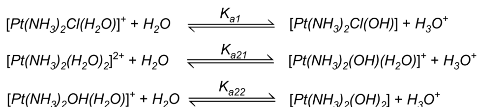
Figure 4 Chemical reactions showing hydrolysis of cisplatin. Reproduced with permission from Burda JV, Zeisinger M, Leszczynski J. Hydration process as an activation of trans- and cisplatin complexes in anticancer treatment. DFT and Ab initio computational study of thermodynamic and kinetic parameters. J Comput Chem. 2005;26(9):907–914. Copyright © 2005 Wiley Periodicals, Inc. 81
