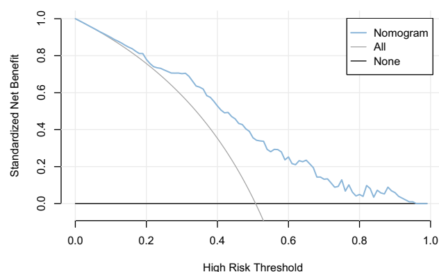
Figure 3 DCA curve analysis of nomogram model.
