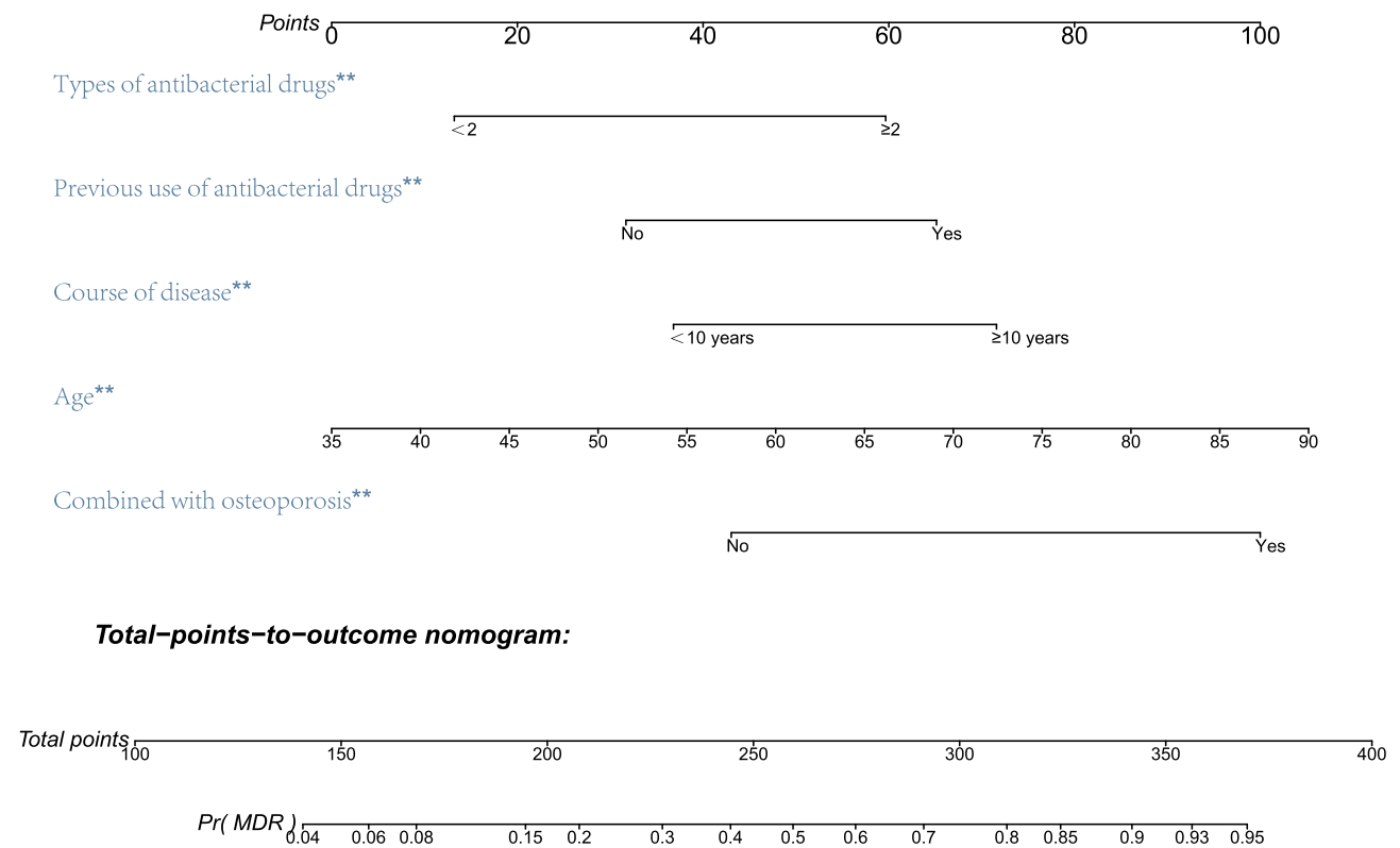
Figure 1 The nomogram model for predicting the risk of MDRB infection in patients with DF. ** P < 0.01 .
