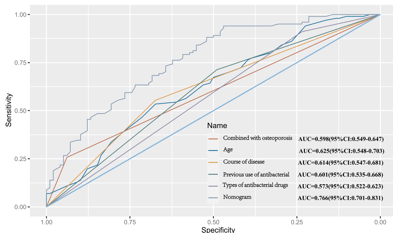
Figure 4 ROC curve analysis of different indicators.
