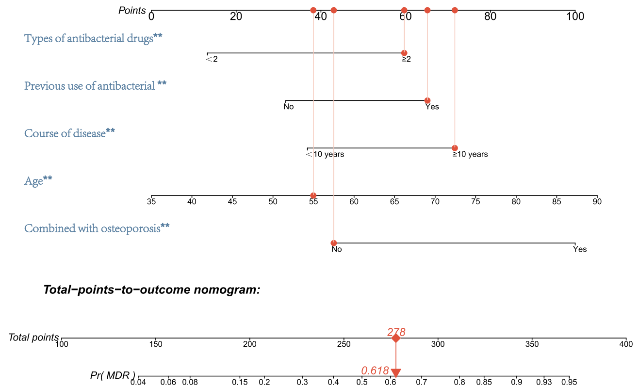
Figure 2 Application example of a nomogram for predicting the risk of MDRB infection in patients with DF. ** P < 0.01 .
