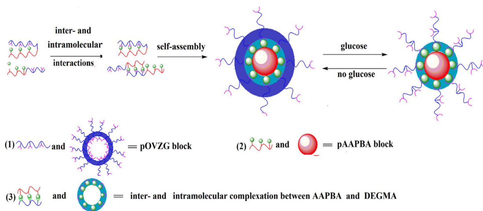
Figure 9 Schematic diagram of the reaction mechanism of p(AAPBA-b-OVZG) nanoparticles to glucose. 78
