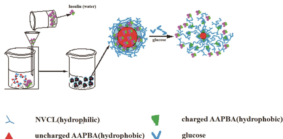
Figure 6 Schematic representation of temperature- and glucose-sensitive p(N-vinylcaprolactam-co-acrylamidophenylboronic acid) p(NVCL-co-AAPBA) nanoparticles. (A) It is a schematic diagram of nanoparticles without insulin; (B) It is a simple schematic diagram of the nanoparticle production process after adding insulin.
