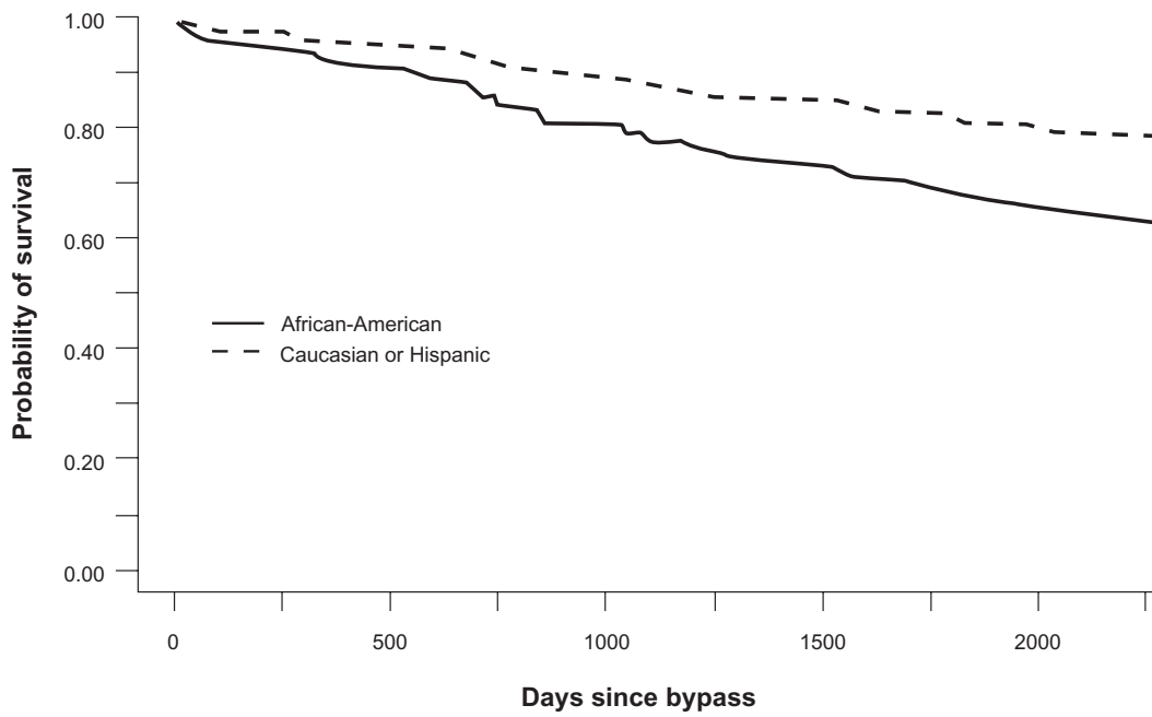
Figure 3 Model-based estimated survival curves for survival after bypass by race/ethnicity.
