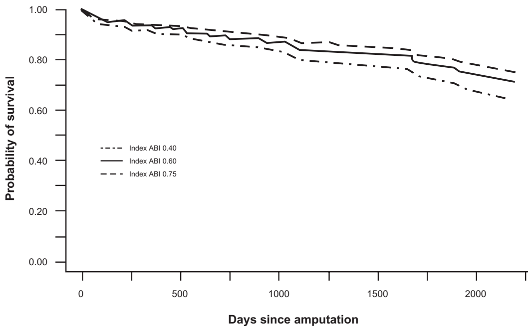
Figure 5 Model-based estimated survival curves for survival after amputation by index ABI. Abbreviation: ABI, ankle-brachial index.
