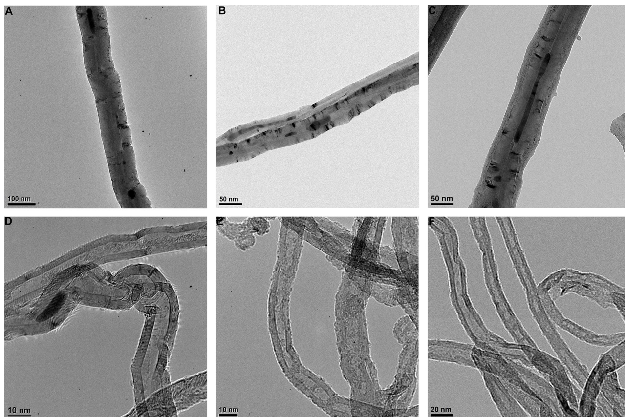
Figure 3 Transmission Electron Microscopy images of (A) pristine MWCNTO, (B) oMWCNTO, (C) oMWCNTN-Sal, (D) pristine MWCNTN, (E) oMWCNTN, and (F) oMWCNTN-Sal.
