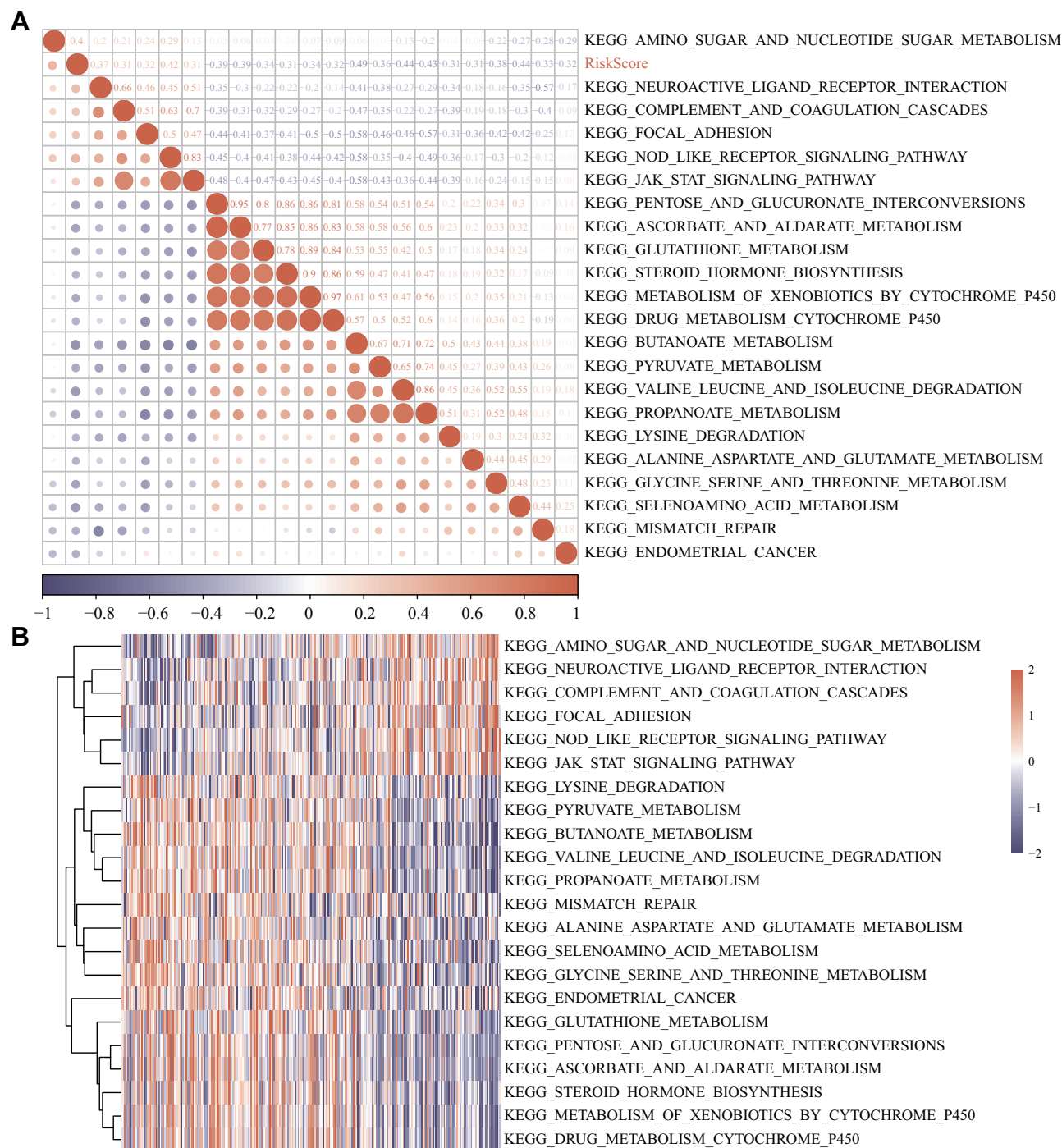
Figure 7 (A) Clustering of correlation coefficients between KEGG pathways with correlation to risk score greater than 0.3 and between risk scores; (B) Changes in ssGSEA scores of KEGG pathways with correlation to risk score greater than 0.33 in each sample, the horizontal axis represents the samples, and the risk scores increase from left to right.
