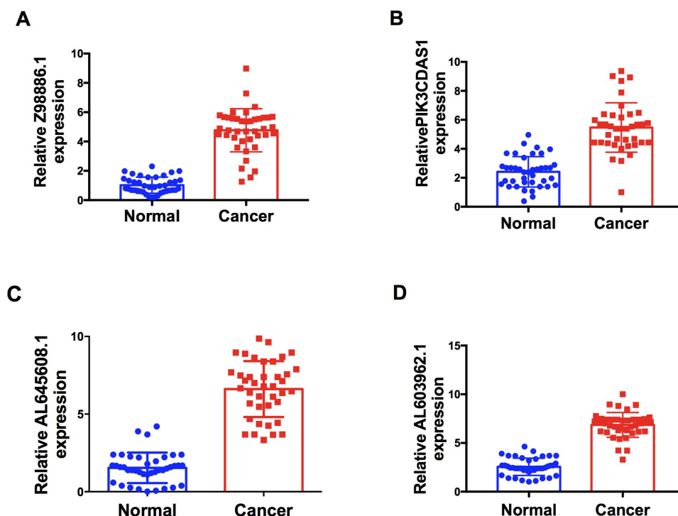
Figure 11 lncRNA levels were validated by reverse transcription quantitative polymerase chain reaction. (A) Z98886.1; (B) PIK3CD-AS1; (C) AL645608.1; (D) AL603962.1. LINC, long non-protein coding RNA between genes; lncRNA, long non-coding RNA.
