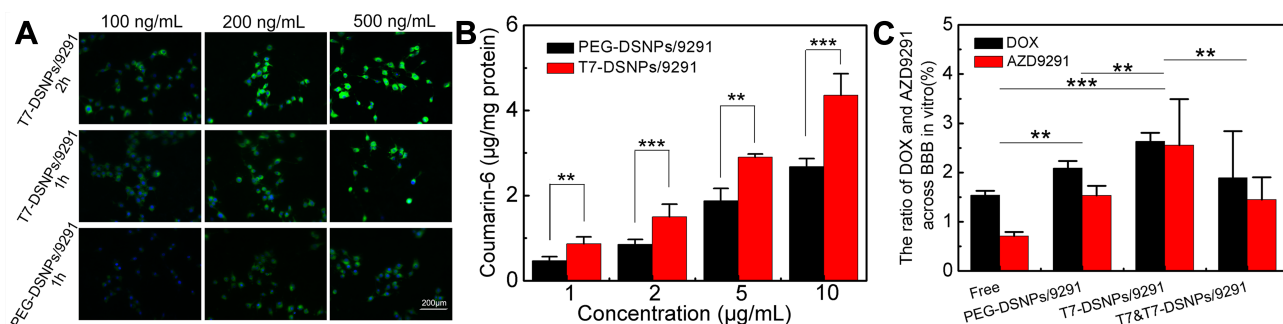
Figure 4 In vitro cellular uptake and penetration capacity of T7-DSNPs/9291. BCEC uptake of T7-DSNPs/9291 and PEG-DSNPs/9291 at 37°C incubated with 100, 200, and 500 ng/mL coumarin-6 for 1 h and 2 h, respectively. Bar: 200 \mu\text{m} (A). BCEC uptake of PEG-DSNPs/9291 and T7-DSNPs/9291 incubated with coumarin-6 concentrations ranged from 1 to 10 \mu\text{g/mL} ( n = 3 ) (B). Trans-BBB transport of AZD9291 and DOX, T7-DSNPs, PEG-DSNPs/9291, and T7-DSNPs/9291 through in vitro BBB model ( n=3 ) (C). *** P < 0.001 , ** P < 0.01 .
