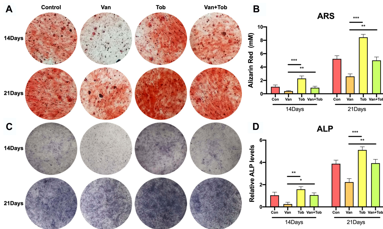
Figure 2 The effect of vancomycin and tobramycin on mineralization of BMSCs was assessed by ARS and ALP staining. BMSCs were stained with ARS and ALP after cultured 14 and 21 days, respectively. ARS staining ( A ) and its quantification ( B ) in the Con, Van, Tob, and Van+Tob groups. ALP staining ( C ) and its quantitative analysis ( D ) in the four groups. * p < 0.05 , ** p < 0.01 , *** p < 0.001 .
