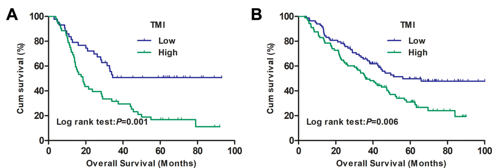
Figure 3 Kaplan-Meier survival analysis according to the TMI level of patients with ESCC who underwent surgery alone ( A , P=0.001 ) and those who underwent surgery with chemotherapy ( B , P=0.006 ).
