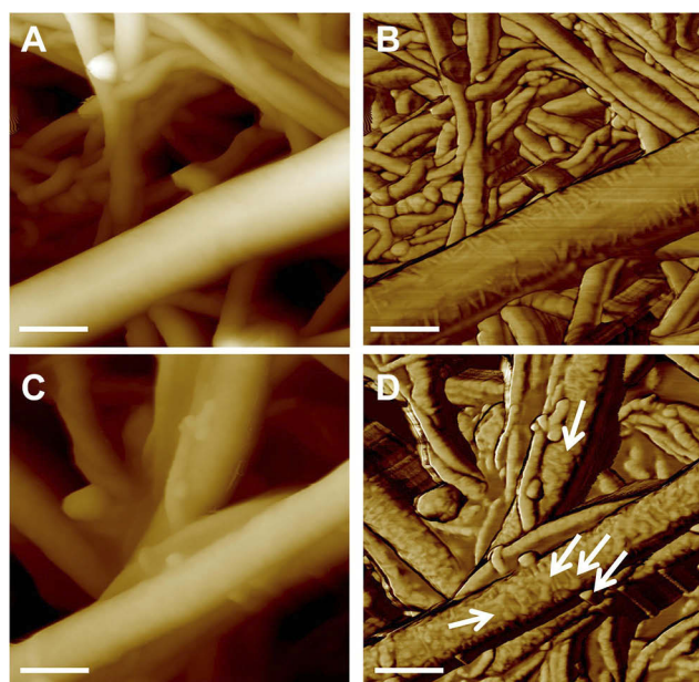
Figure 2 Height (left) and phase (right) channels by AFM measurements of the pristine buckypaper (A, B) and of the PAMAM-coated one (C, D). Arrows in panel D indicate the small bubble-like structures of the polymer coating the BP surface (D). In all panels, scale bar is 200 nm.
