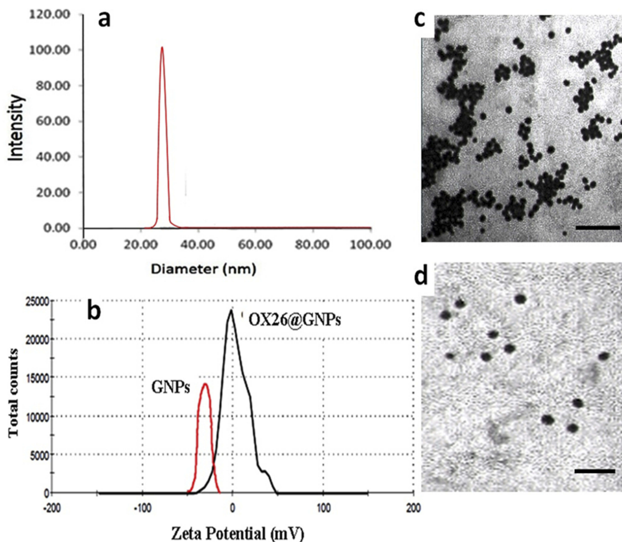
Figure 2 Physicochemical characterization of GNP. (A) Particle size analysis of OX26@GNPs using dynamic light scattering (DLS), (B) Zeta potential distribution of GNP along with OX26@GNPs. TEM images of (C) GNP (scale bar 200 nm) and (D) OX26@GNPs (scale bar 100 nm).
