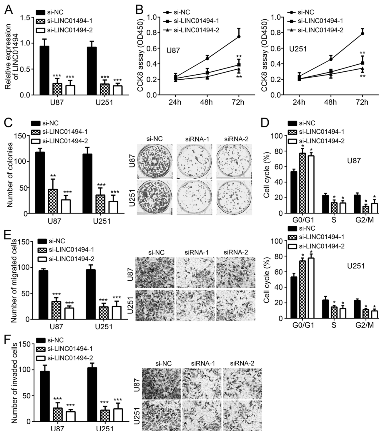
Figure 2 Effects of LINC01494 knockdown on glioma proliferation, migration and invasion. (A) Two independent siRNAs against LINC01494 were transfected into U87 and U251 cells and the efficiency of LINC01494 knockdown was confirmed. (B) CCK8 assay was performed to test cellular proliferation. (C) LINC01494 knockdown led to reduced colony numbers. (D) The effect of LINC01494 knockdown on cell cycle was analyzed by FACS. (E and F) LINC01494 knockdown suppressed the migration and invasion of U87 and U251 cells. * P < 0.05 , ** P < 0.01 and *** P < 0.001 .
