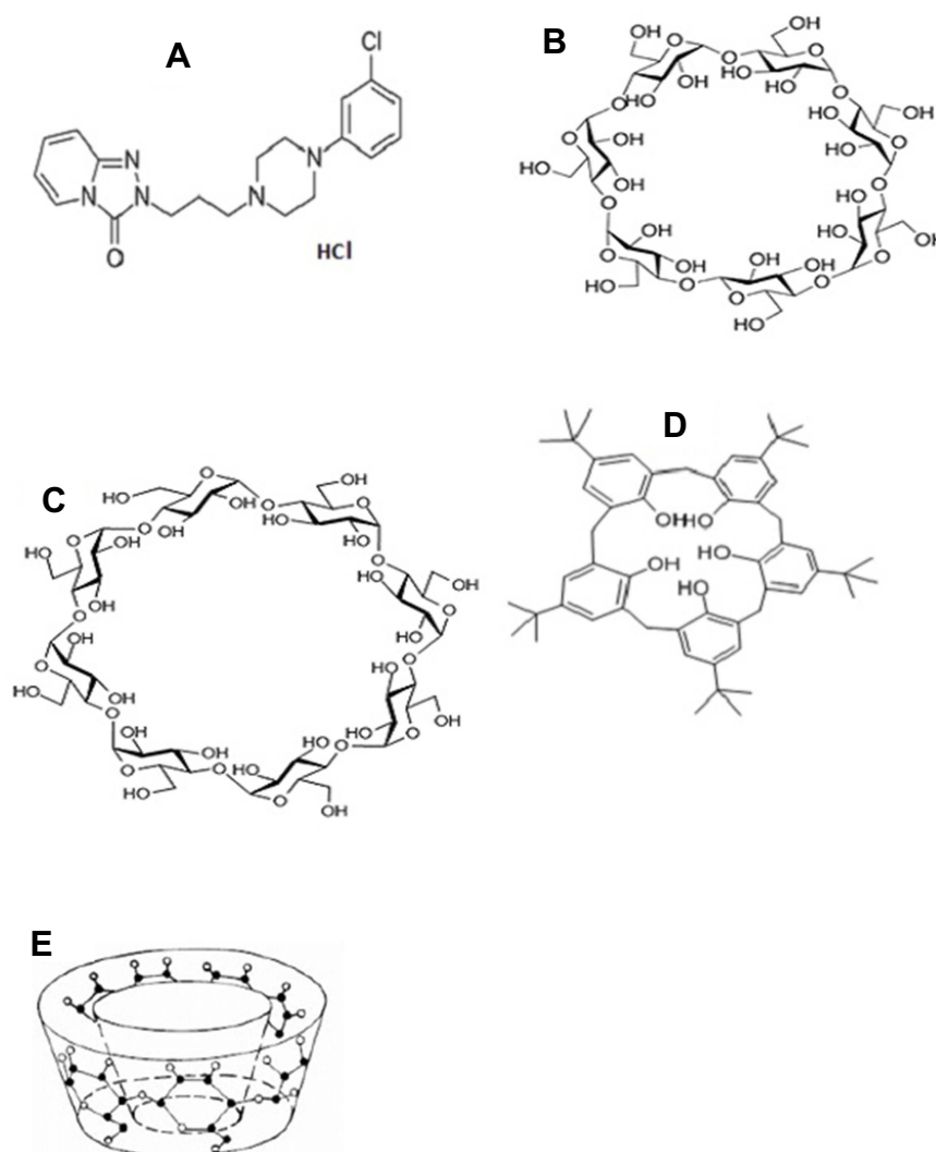
Figure 1 Chemical structures of trazodone (A), β-CD (B), γ-CD (C), 4t-BC8 (D), and the toroidal shape (E).
