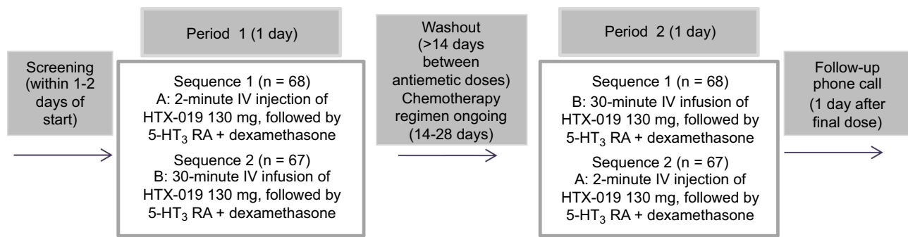
Figure 1 Study design.
