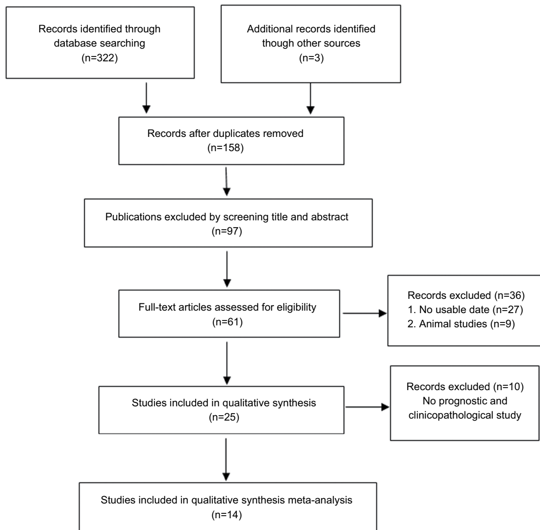
Figure 1 Flow diagram of literature search and selection.
