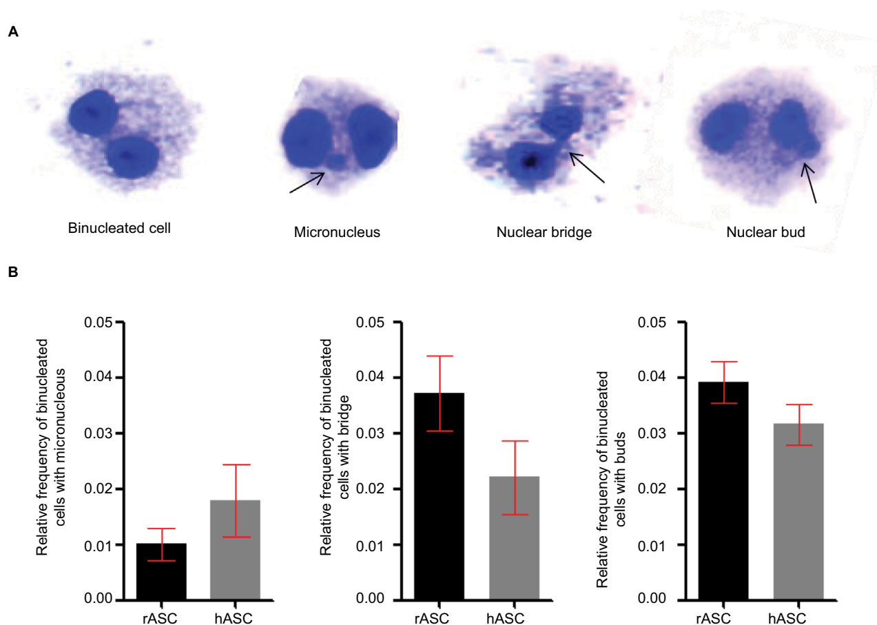
Figure 3 Nuclear stability.
