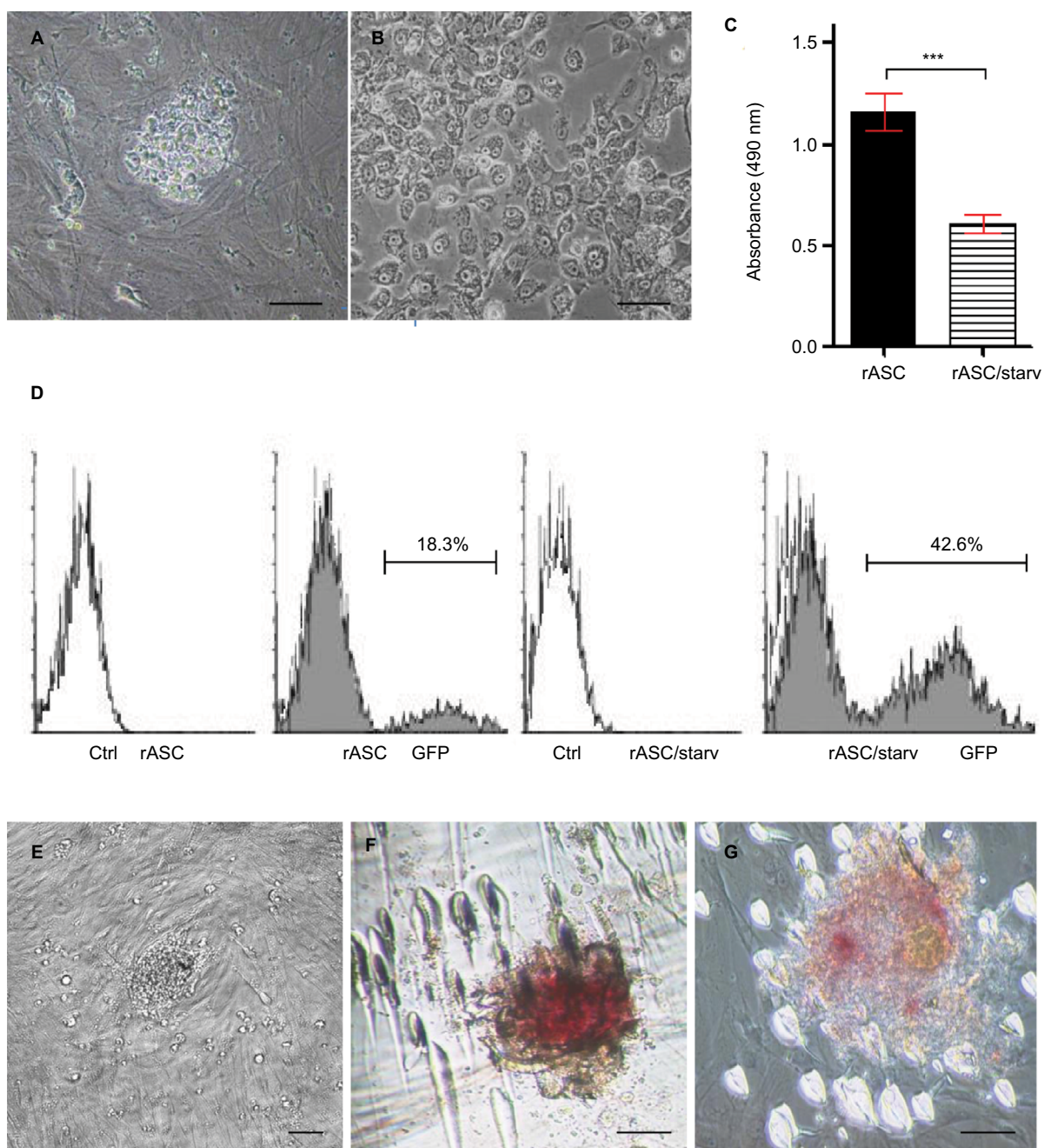
Figure S1 Induction of pluripotency in rASCs.
