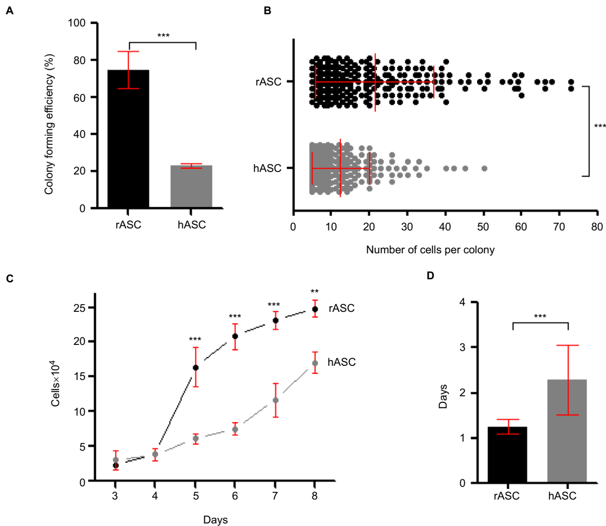
Figure 2 Proliferative profile of rASCs vs hASCs.
