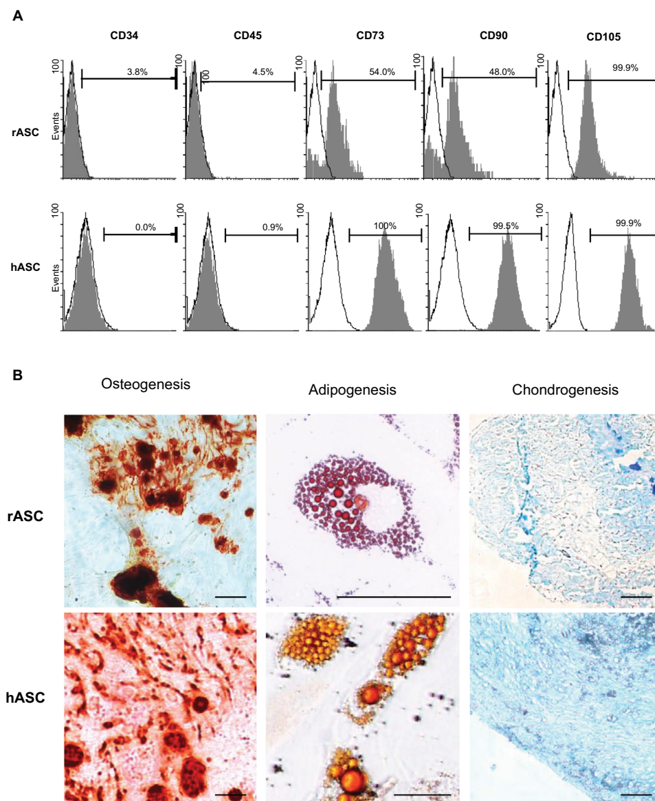
Figure 1 Stemness characterization.
