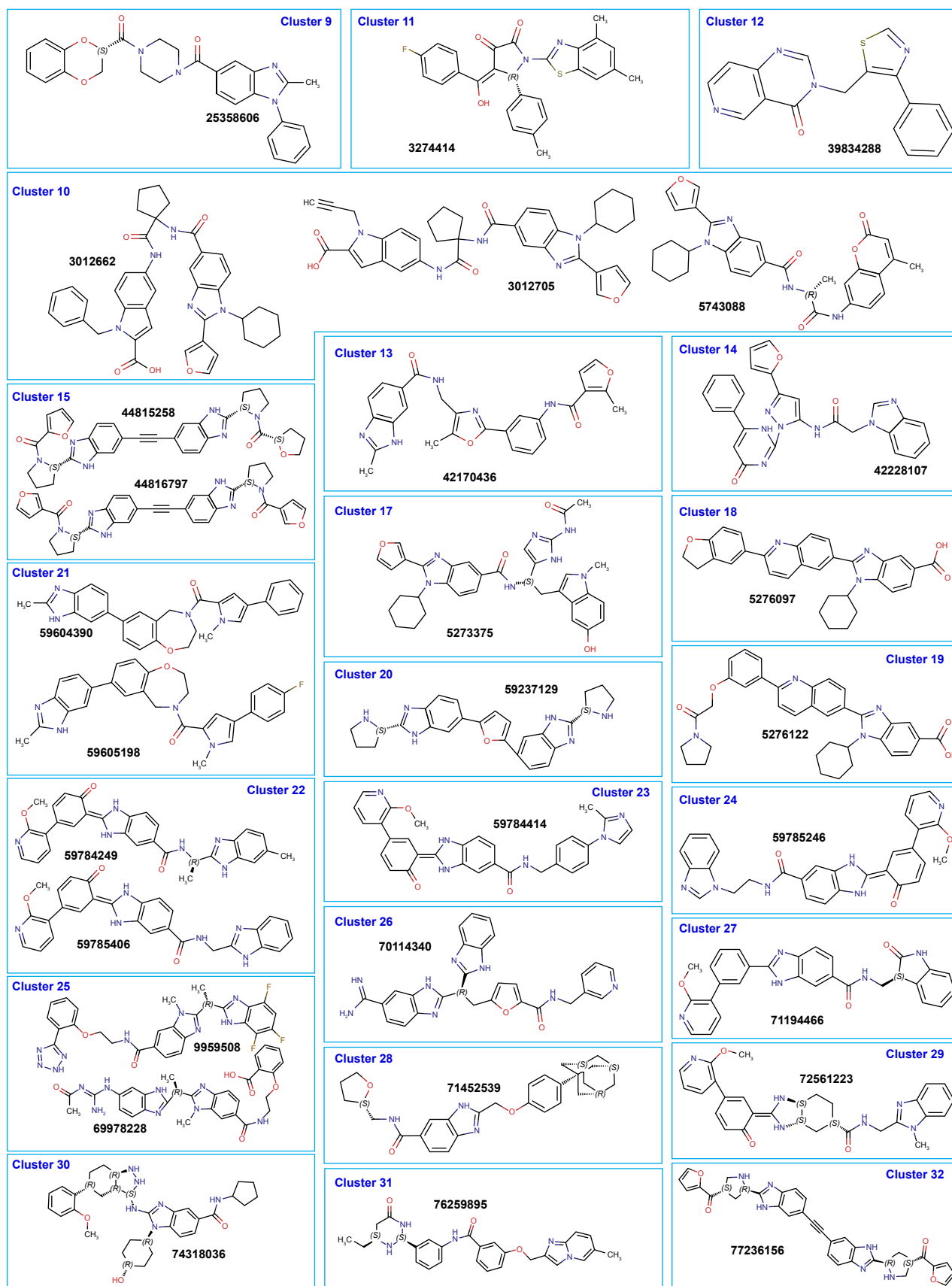
Figure S1 Molecular structure of compounds selected against the allosteric binding site for HCV NS5B (A) and IPNV VPI RdRp (B).
