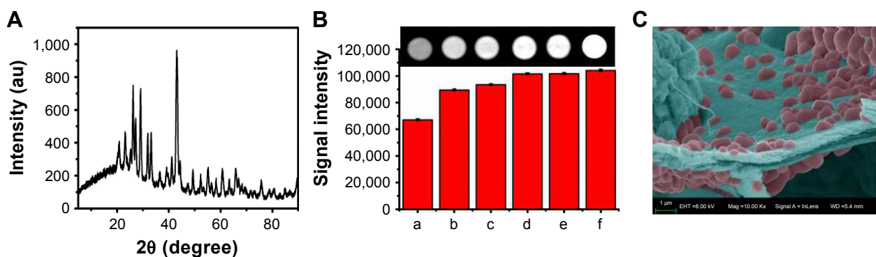
Figure 2 (A) XRD patterns of CA/BaSO 4 microcapsules measured with 2θ ranging from 5° to 90.0° in a step of 0.02° under a Cu Kα radiation. (B) CT images of CA/BaSO 4 microcapsules using various concentrations of Na 2 SO 4 as injection liquid arranged from 0 mg/mL to 7.5 mg/mL (b–e: 0, 2.5, 5, 7.5 mg/mL); phosphate buffered saline was used as the negative control (a) and iodixanol solution was used as the positive control (f). (C) SEM images of barium sulfate nanoclusters.
