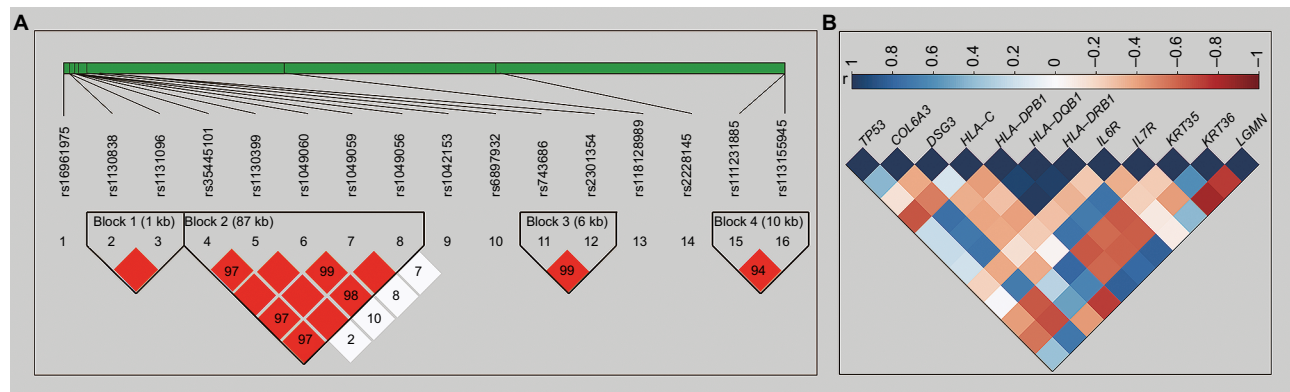
Figure 1 Haplotype association of the candidate SNPs and co-expression heat map for the TP53 gene and corresponding genes of the candidate SNPs.
