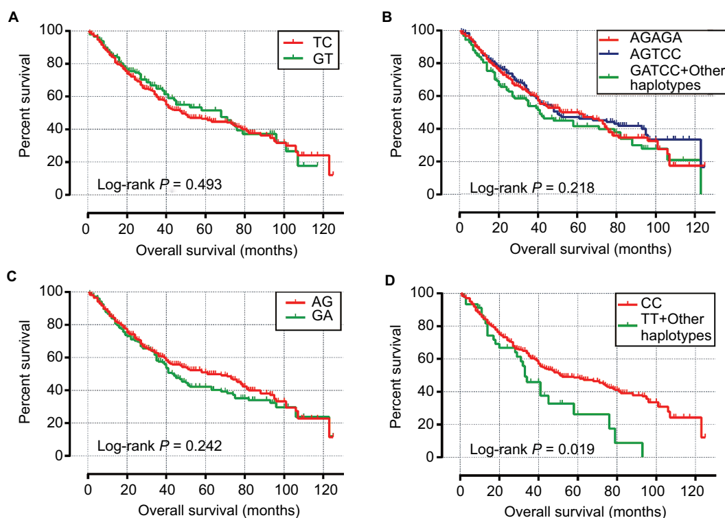
Figure 5 Survival curves of different haplotypes.
