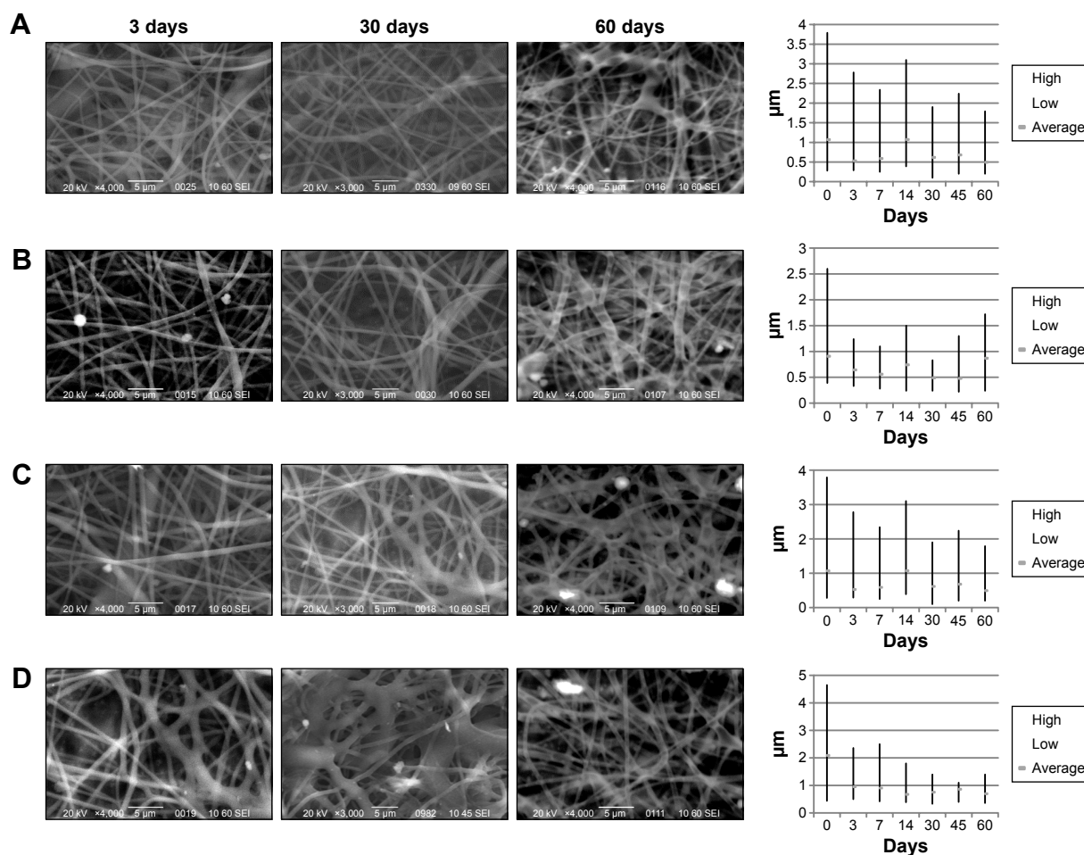
Figure 7 SEM images and diagrams of biodegradation of (A) 14%, (B) 16%, (C) 18%, and (D) 20% AC drug-loaded nanofibers at 3, 30, and 60 days.
