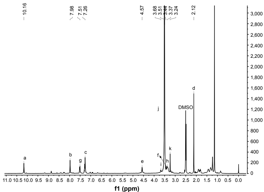
Figure S3 ^1\text{H} -NMR spectrum of MPEG-PHIS.
