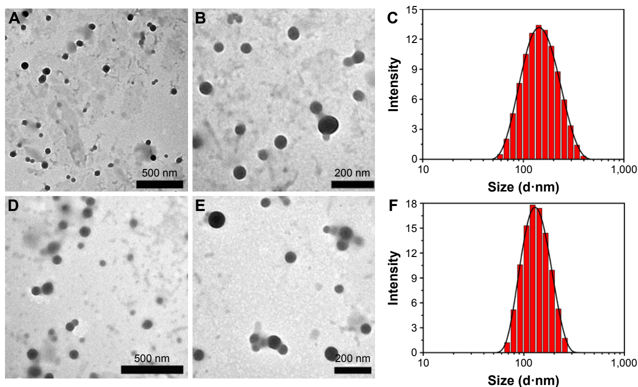
Figure 3 TEM image and size distribution of DOX-loaded Z_1 /CMCS 1 -TA/Cu 2+ NPs (A–C) and Z_1 /CMCS 1 -TA/Ca 2+ (D–F). The Z_1 /CMCS 1 NPs were prepared at zein:CMCS ratio of 1:1 w/w with the final metal ion concentration of 0.24 mM (Cu 2+ or Ca 2+ ).
