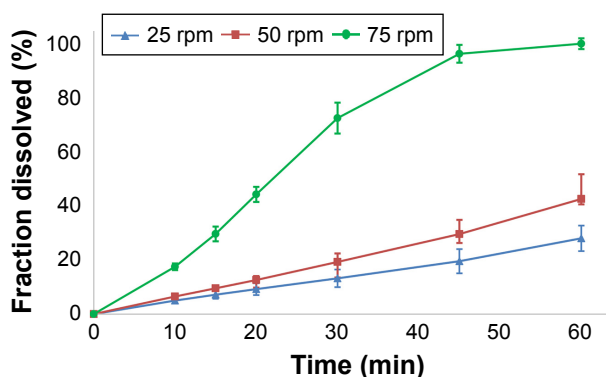
Figure 7 Dissolution of SET formulation (500 mg drug loading) in acetate buffer pH 4.5 at various paddle speeds.
