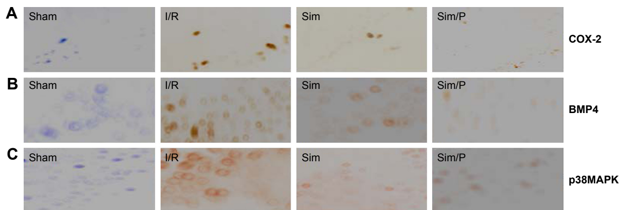
Figure 8 Expression of COX-2 (A), BMP4 (B), and p38MAPK (C) in different groups of rats.
