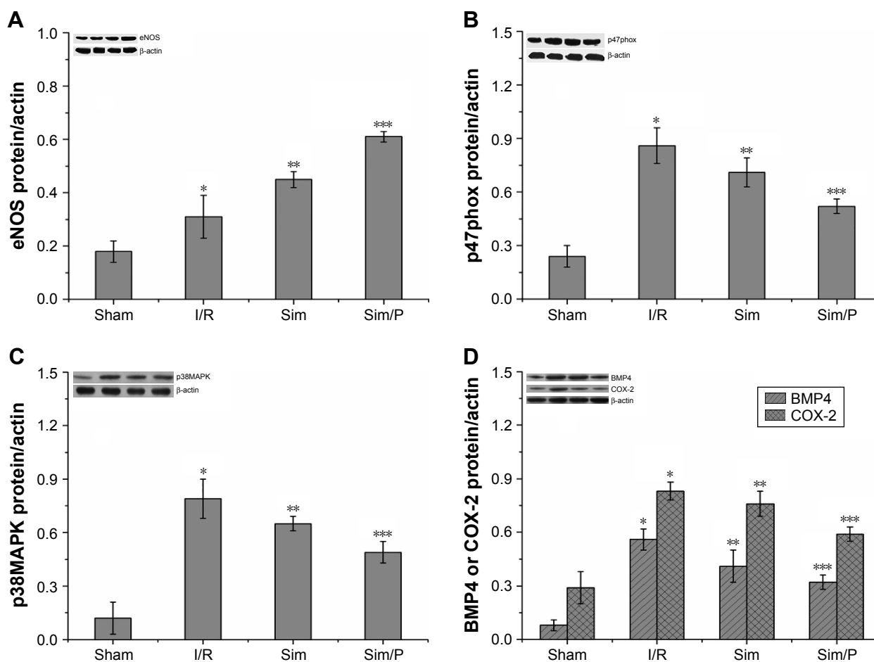
Figure 7 Expression of eNOS (A), p47phox (B), p38MAPK (C), BMP4, and COX-2 (D) in different groups of rats.
