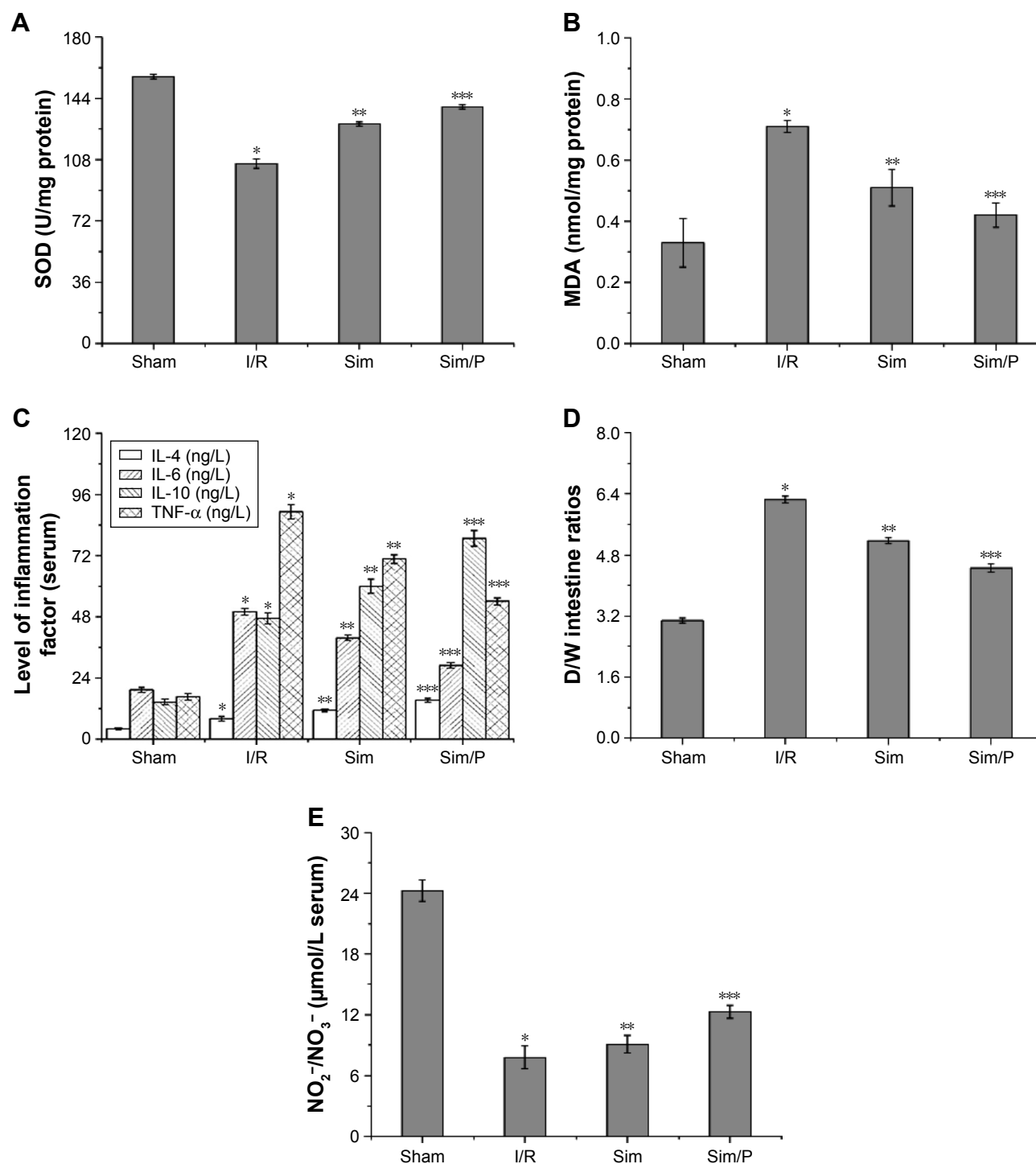
Figure 5 (A) SOD activity; (B) MDA level; (C) Level of IL-4, IL-6, IL-10, and TNF-α; (D) D/W intestine ratios; (E) Level of serum NO 2 - /NO 3 - .
