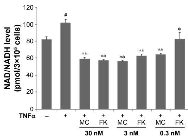
Figure 5 Inhibitory effects of MC4 and FK866 on TNF \alpha -induced intracellular NAD/NADH levels in A549 cells.
