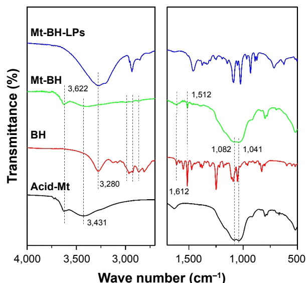
Figure 8 FTIR spectra of acid-Mt, BH, Mt-BH, and Mt-BH-LPs.
