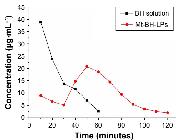
Figure 16 Concentration–time curve in the cornea/tear-film compartment after topical application of BH solution and Mt-BH-LPs.
