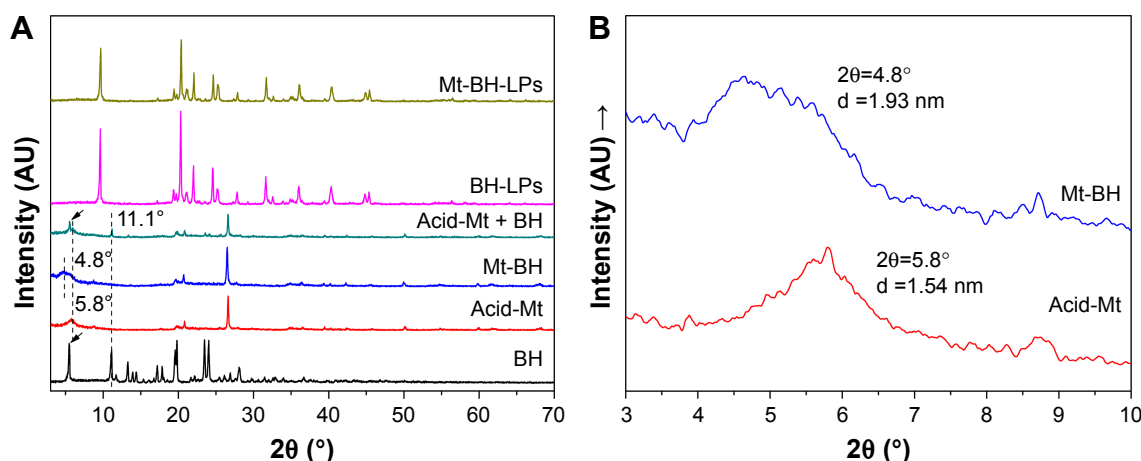
Figure 6 (A) XRD patterns of BH, acid-Mt, Mt-BH, acid-Mt + BH, BH-LPs, and Mt-BH-LPs; (B) enlarged XRD patterns of acid-Mt and Mt-BH.
