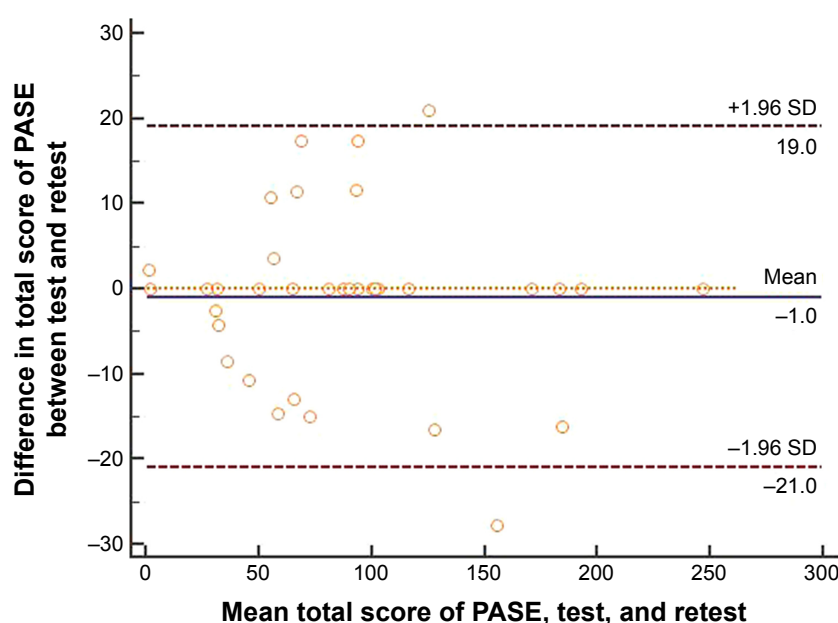
Figure 1 Bland–Altman plot for total score of PASE.
