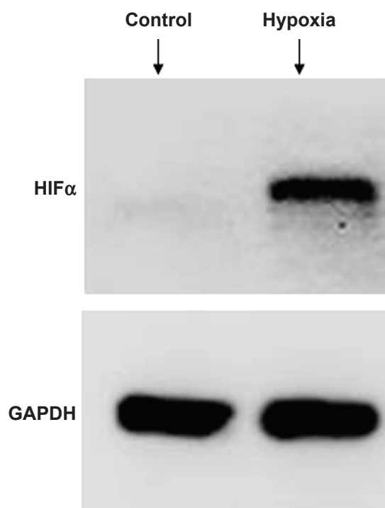
Figure 1 Expression of HIFα in A549 cells detected by Western blot analysis. Notes: "Control" represents the group of A549 cells cultured in the normoxic condition, and "hypoxia" represents the group of A549 cells cultured in a hypoxia incubator (1% O 2 ). Abbreviations: HIFα, hypoxia-inducible factor α; GAPDH, glyceraldehyde-3-phosphate dehydrogenase.
