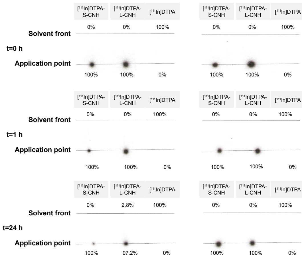
Figure S3 TLC papers showing the radiolabeling stability of [^{111}\text{In}]\text{DTPA-S-CNH} s and [^{111}\text{In}]\text{DTPA-L-CNH} s in mouse serum (left column) and PBS (right column) over 24 hours (h).
