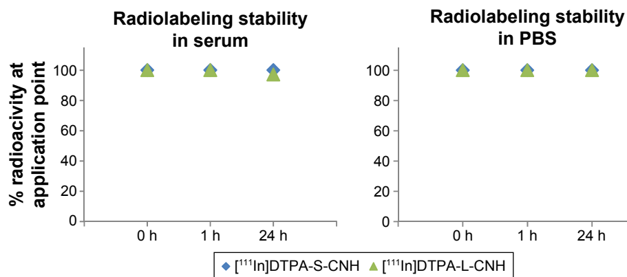
Figure S4 Radiolabeling stability of [^{111}\text{In}]\text{DTPA-S-CNH} s and [^{111}\text{In}]\text{DTPA-L-CNH} s in mouse serum (left) and PBS (right) over 24 hours (h).
