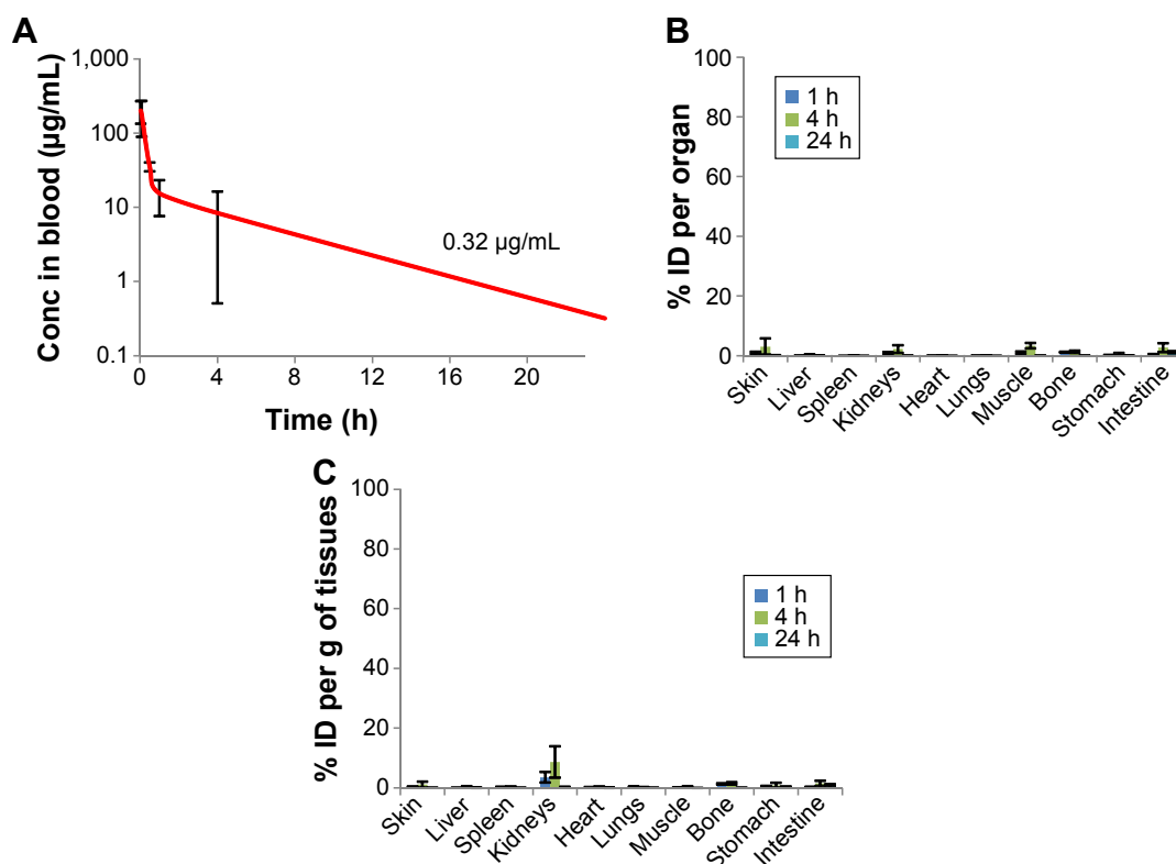
Figure S6 Quantities of [ ^{111}\text{In} ]DTPA control injected intravenously in mice detected by gamma scintigraphy up to 24 hours (h) postinjection.
