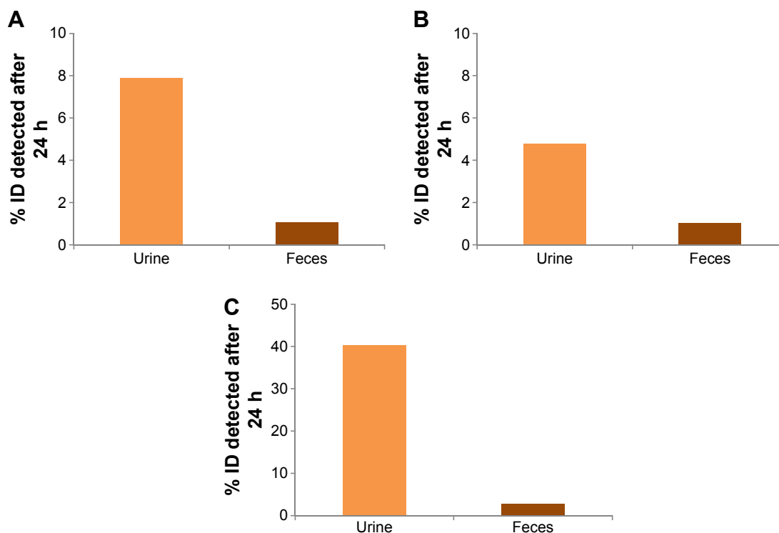
Figure S7 Metabolic profile represented by amounts of [ ^{111}\text{In} ] labeled S- or L-CNHs (% ID) detected in urine and feces 24 hours postinjection.
