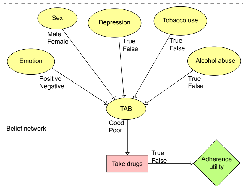
Figure 3 A Bayesian decision network for predicting TB TAB.
