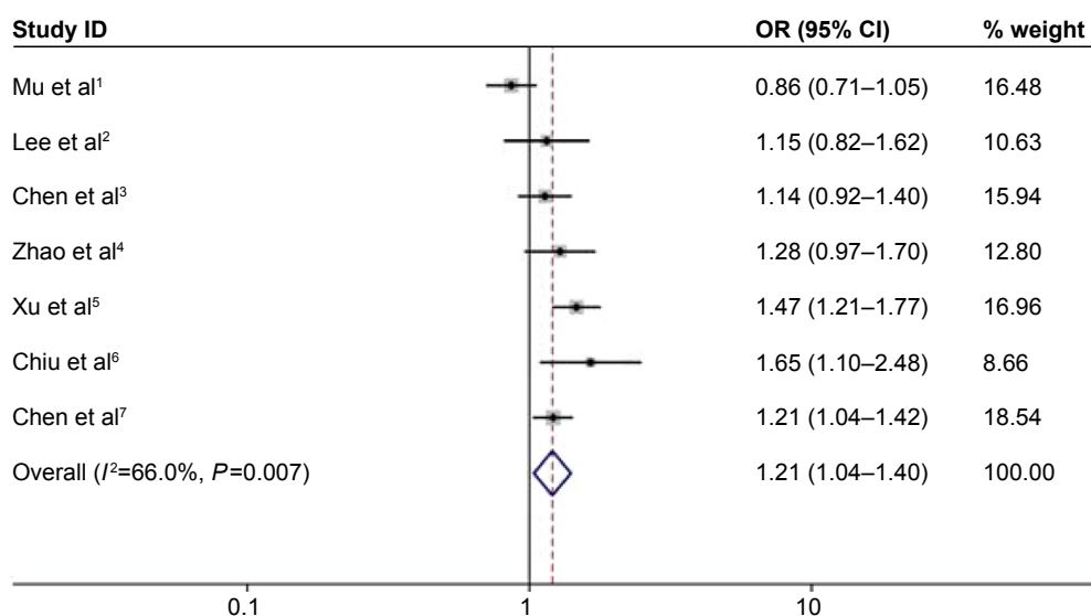
Figure S1 Forest plot for the association between OPN rs17524488 (-156-/G) polymorphism and cancer risk (G allele vs - allele).
