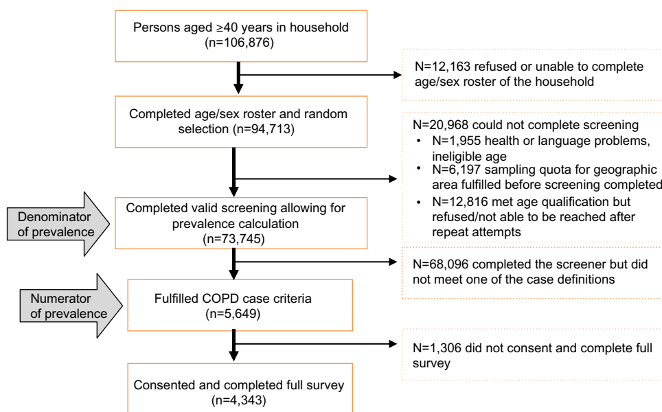
Figure 1 Study-consort diagram.
