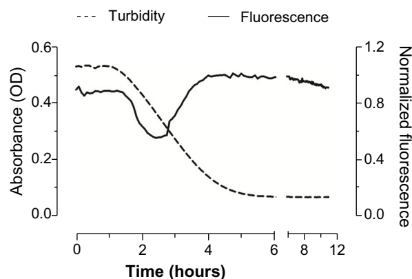
Figure 4 Variation of turbidity (absorbance at \lambda 510 nm) and fluorescence (excitation \lambda 350 nm, emission \lambda 670 nm) with time for AlPc-NPs (1 \mu M AlPc) dispersed in PBS at 25°C.
