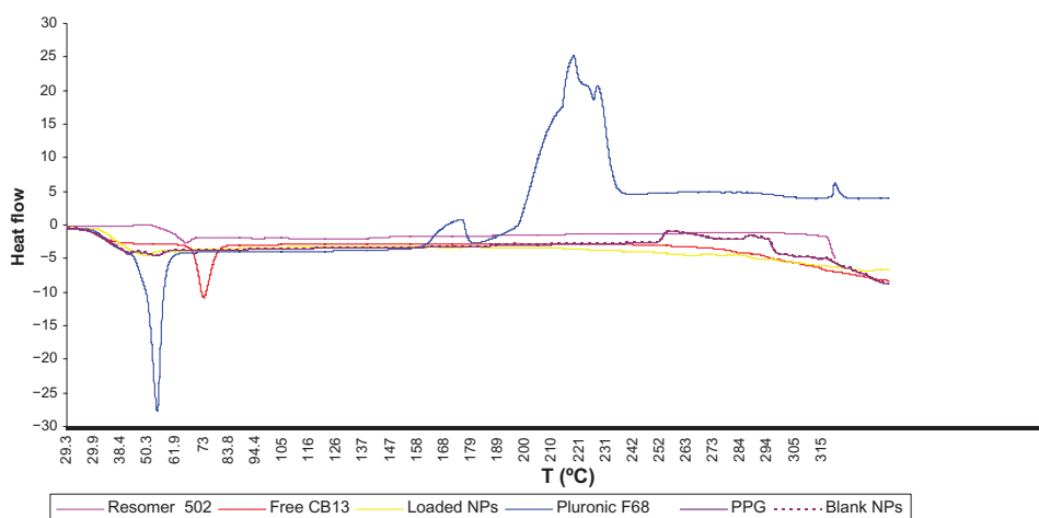
Figure 2 DSC curves of Resomer 502, free CB13, loaded-PLGA NPs (20% w/w), Pluronic® F68, PPG, and blank-PLGA NPs.
